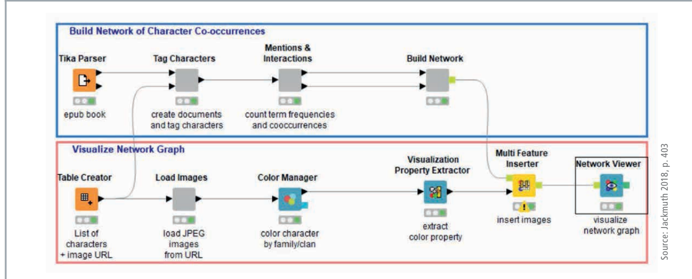
Fig. 02: Extract from the KNIME workflow
