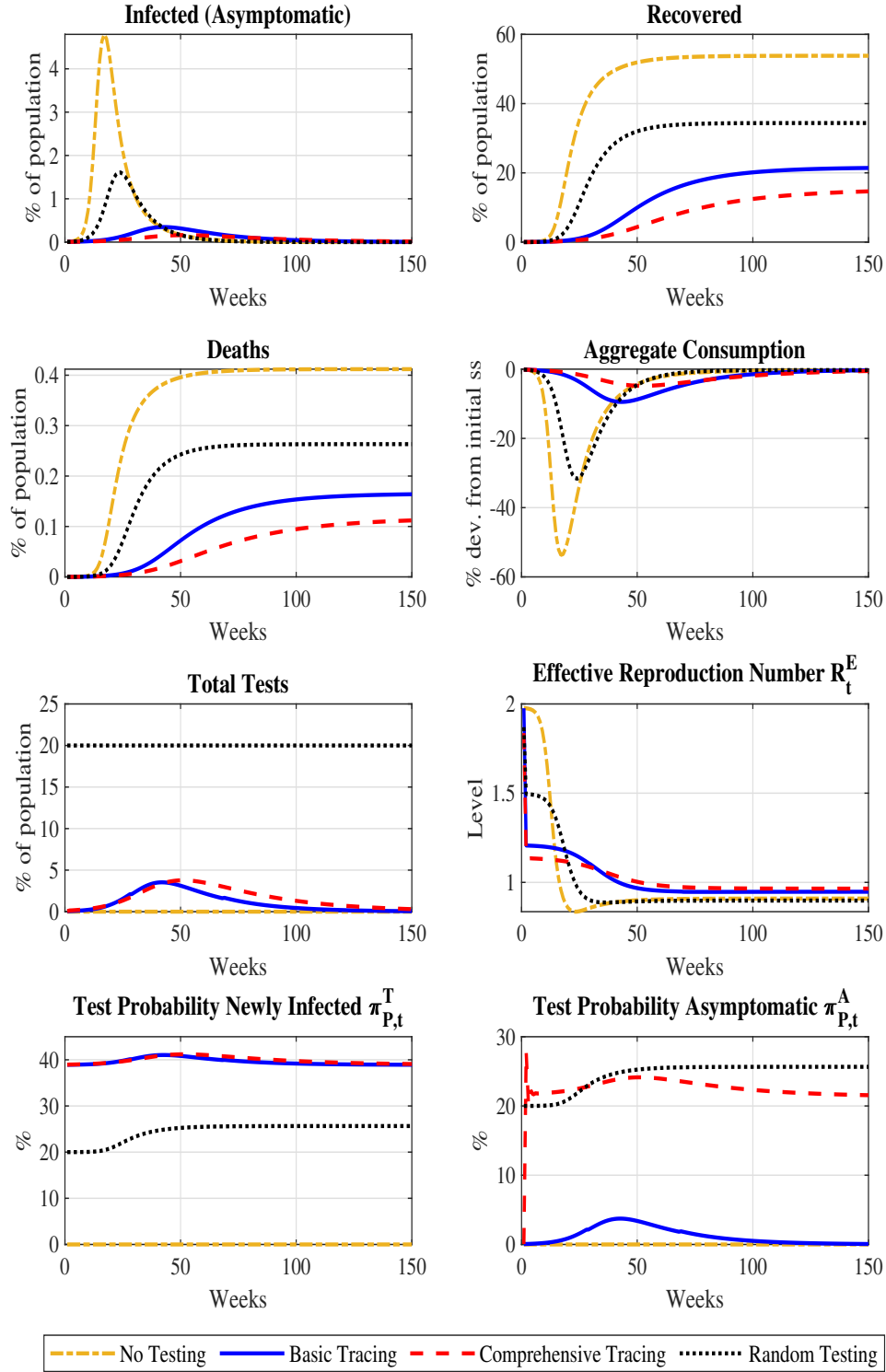
Figure 2: Comparison of different testing strategies with unconstrained number of tests for contact tracing. We assume that the amount tests available for random testing is 20% of the entire population each week.
