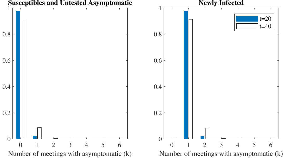
Figure 11: Probability distributions for an agent who does not know their health status to meet with untested asymptomatic subjects k times. The left plot graphs the distribution f_t(k) defined in equation (22) and concerns susceptible agents, who do not turn out to become infected in the period, untested asymptomatic agents, and unobserved recovered agents. The right plot graphs the distribution f_t^T(k) obtained by applying the Bayes theorem as shown in equation (24) and concerns the newly infected agents. The distributions are obtained in period 20 (blue bars) and 40 (white bars) of the simulation in which we assume basic tracing technology and unlimited testing capacity (Section 5.1).
