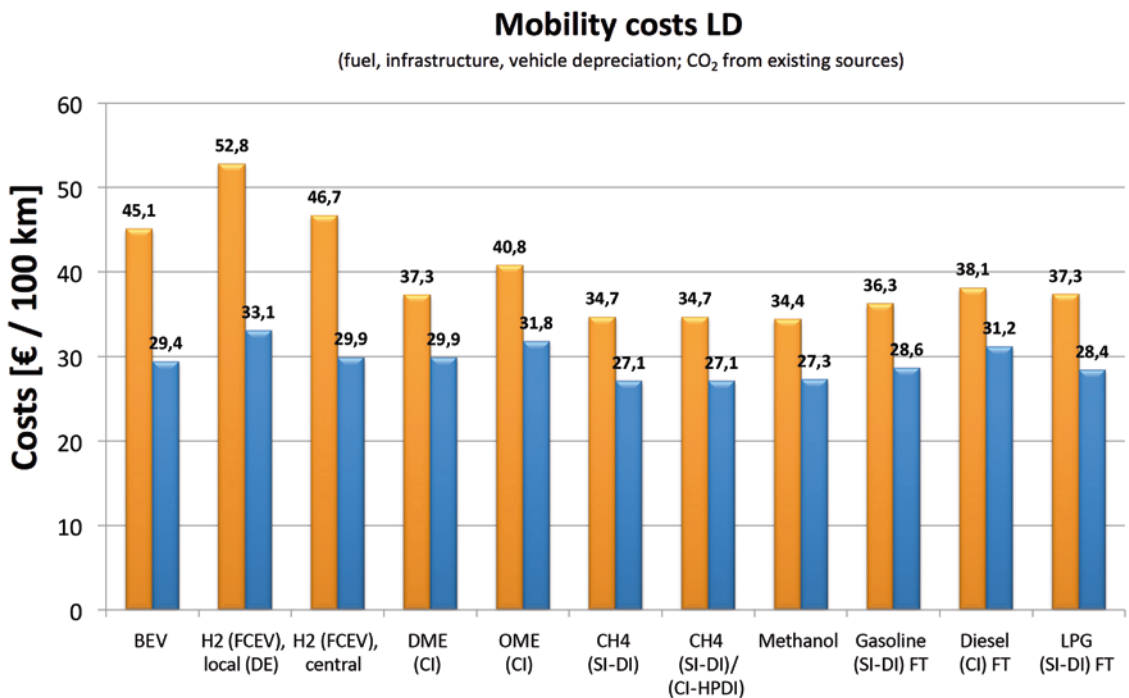
Figure 25: Min./max. mobility costs for cars [€/100 km] – framework conditions as per Table 12, but without taking into account the energy requirement for CO 2 separation (assumption: CO 2 from existing sources)
