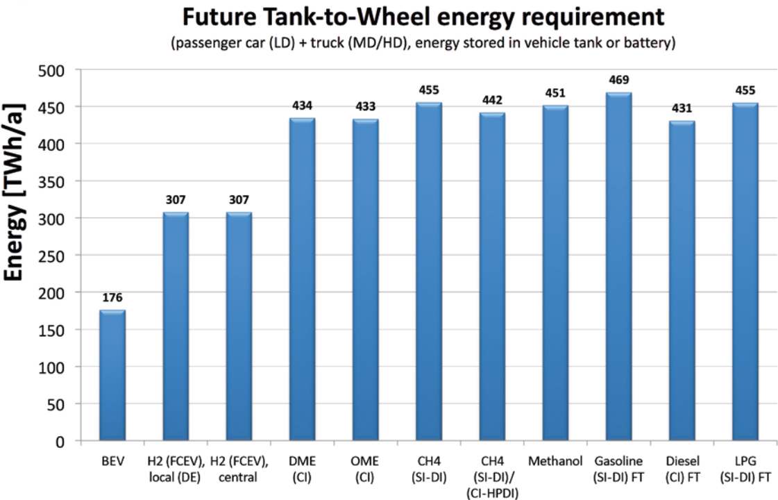
Figure 6: TtW energy requirement [TWh/a]
