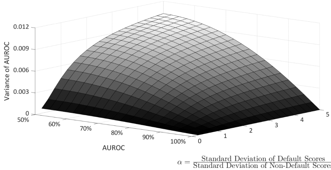
Figure 10: Variance of the AUROC for normally distributed credit scores (with \sigma = 3 ) as a function of the AUROC and the parameter \alpha for a synthetic data set of 1,000 obligors.
