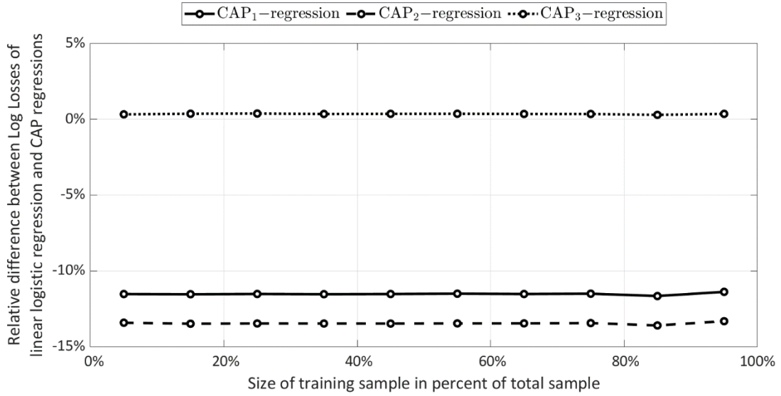
Figure 6: Medians of relative differences in Log Loss between linear logistic regression and CAP regressions as functions of the training sample size.
