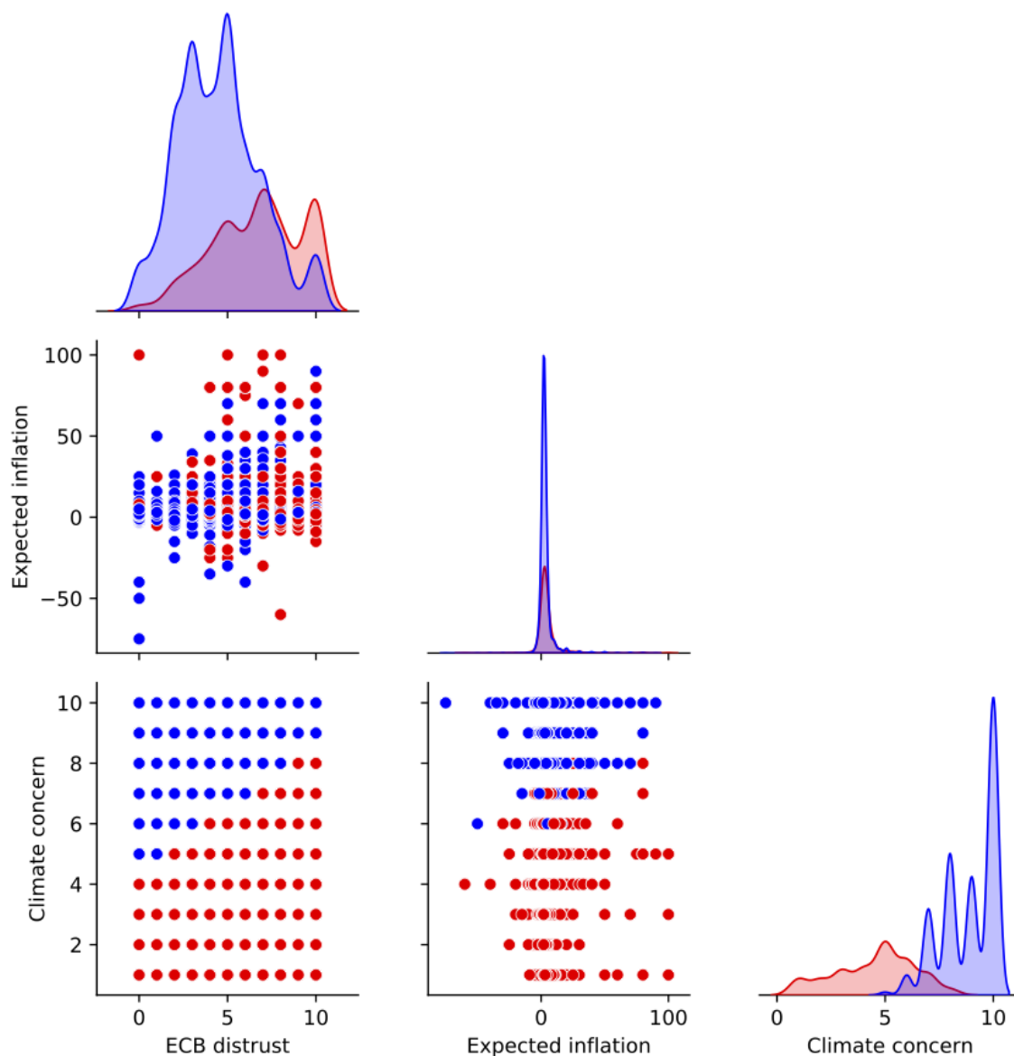
Figure 2: Pairplot
