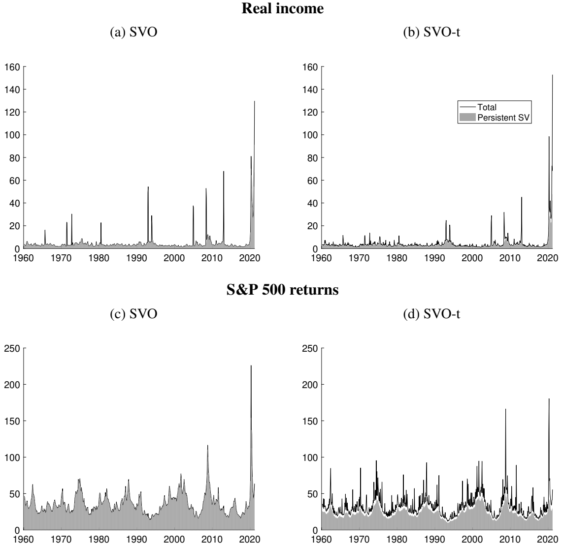
Figure 1: Contributions of outlier adjustments to forecast-error volatilities
