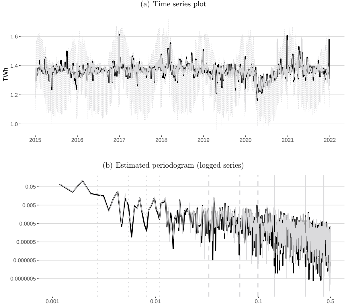
Figure 6: Seasonally adjusted electricity consumption obtained from the extended X-11 ( black ) and AMB ( grey ) approaches. Dashed grey line in Panel (a) corresponds to unadjusted series. Grey verticals in Panel (b) correspond to selected seasonal harmonics of the DOY ( dotted ), DOM ( dashed ) and DOW ( solid ) patterns.
