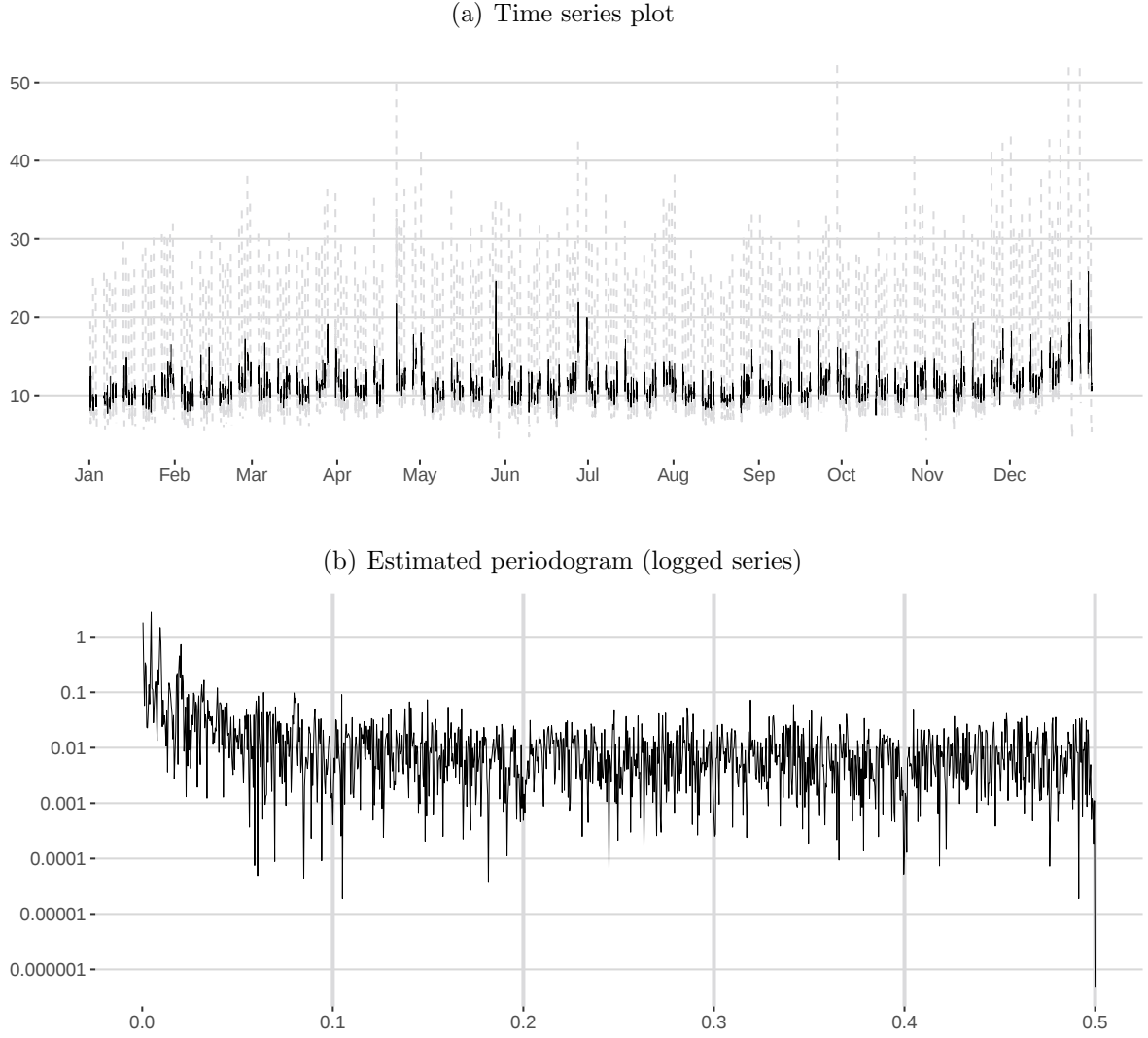
Figure 10: Seasonally adjusted HCP series obtained from the STS approach. Dashed line in Panel (a) corresponds to unadjusted series. Grey verticals in Panel (b) correspond to HOD harmonics.
