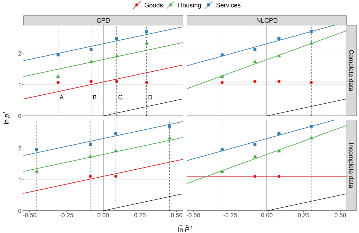
Figure 1: CPD and NLCPD regressions for the price data of Tab. 1, either with complete price data (top panels) or with missing prices for “goods” (bottom panels).
