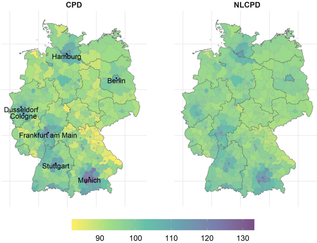
Figure 4: Price index numbers by CPD and NLCPD methods, each in relation to its population-weighted average (= 100).
