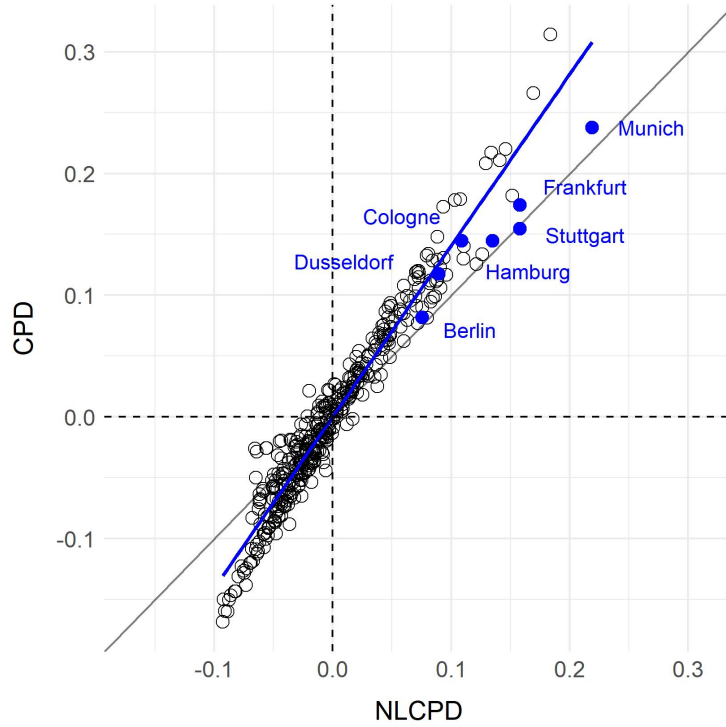
Figure 3: Estimates of the regional logarithmic price levels, \ln P^r , by NLCPD method (horizontal axis) and CPD method (vertical axis). Ordinary least squares regression as solid blue line.
