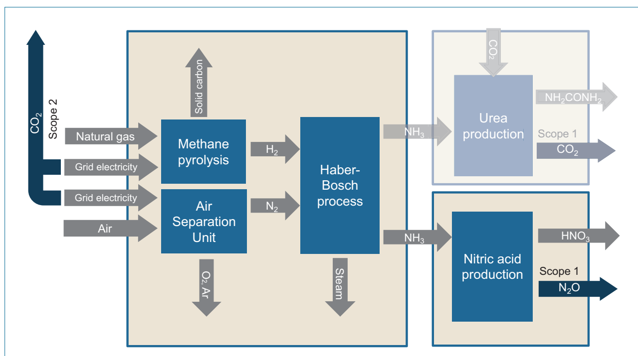
Figure 3.6 Methane pyrolysis (turquoise hydrogen)
