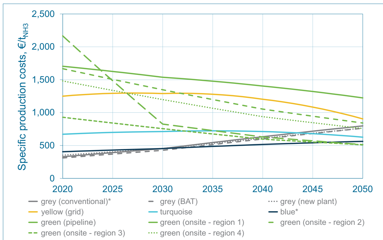
Figure 5.5 Specific production costs of ammonia, non-depreciated, full implementation of technologies.
