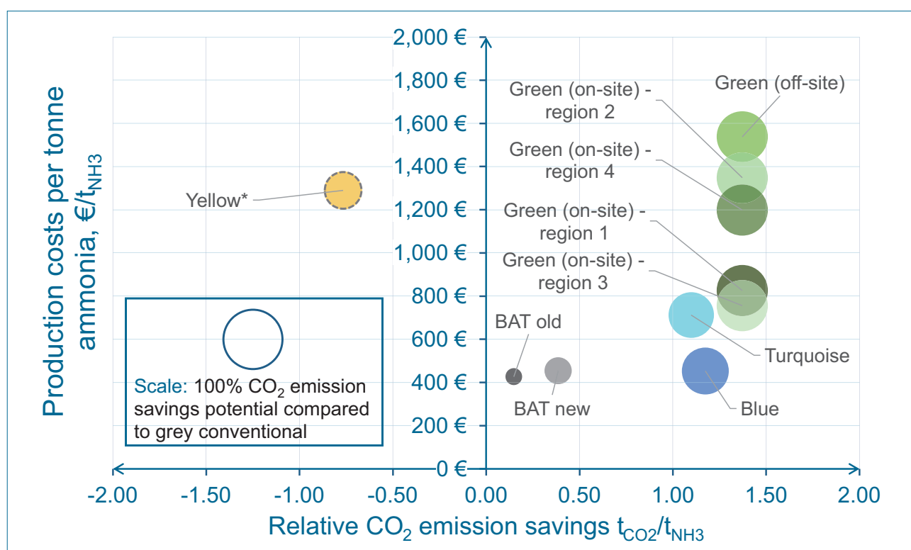
Figure 5.7 Production costs vs. relative CO 2 -emission savings of different technologies in 2030 compared to grey conventional.
