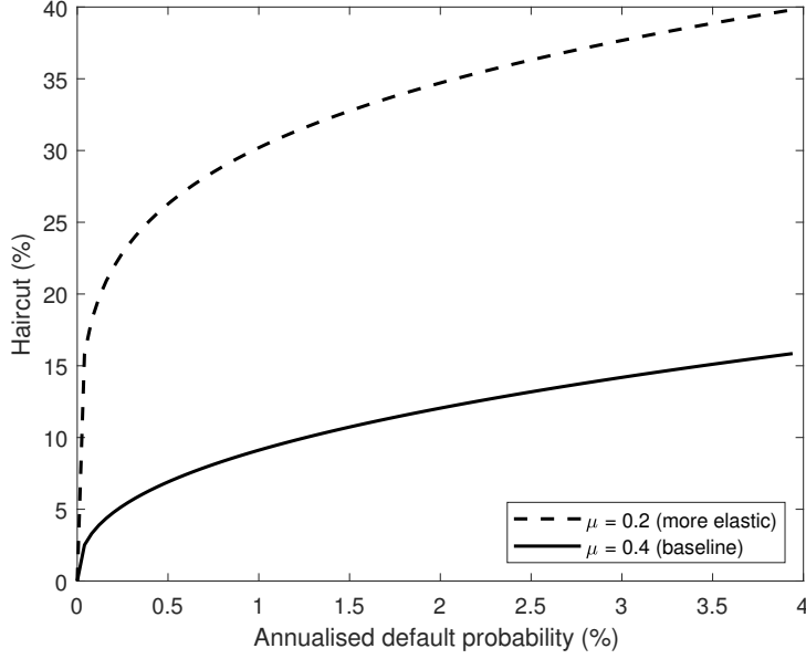
Figure 2: Haircut function
