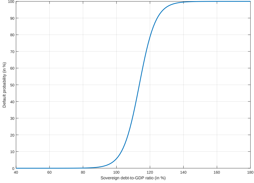
Figure 2: Default Probability
