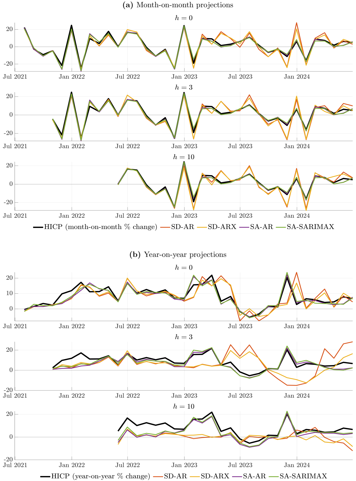
Figure 4: Realised HICP-PACK and projections at horizons h = 0, 3, 10
