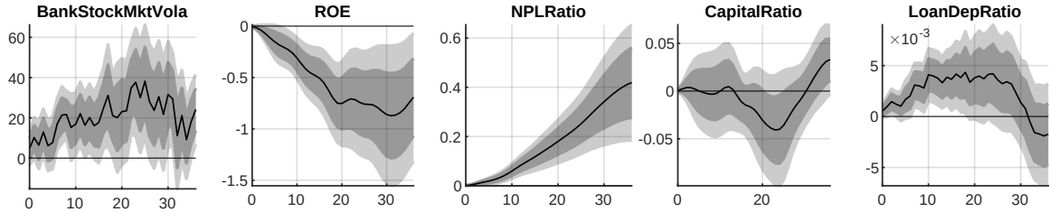
Figure 8: Impulse responses of bank risk
