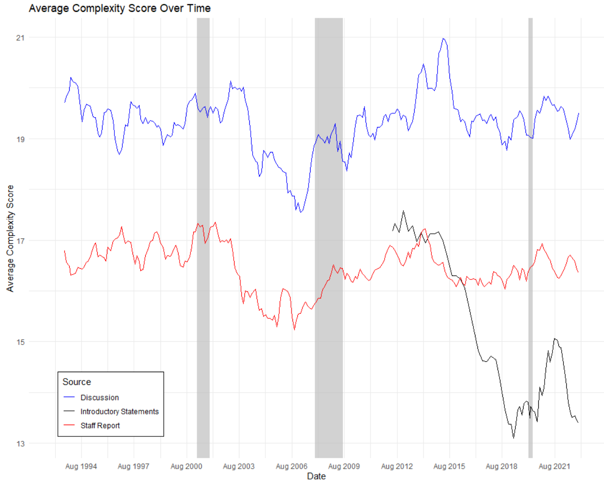
Figure 1: Complexity Measures for FOMC Documents 01.1993-12.2018
