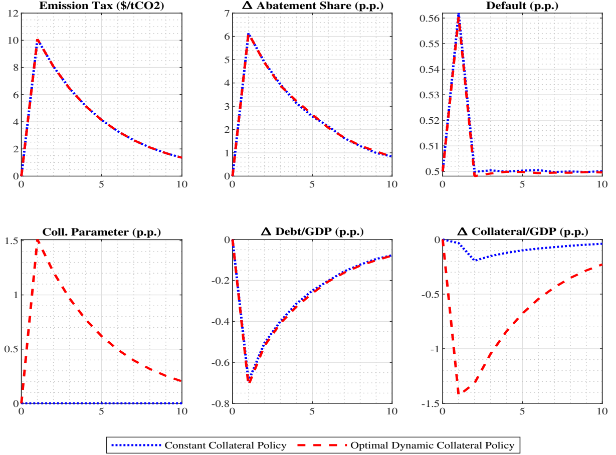
Figure 3: IRF to 10$/tCO2 Emission Tax Shock. This figure displays the impulse response to a 10$/tCO2 emission tax shock on key macro-financial variables. The top row displays the change in the share of abated emissions \nu_t^* and the corporate default rate F(\bar{m}_t) , both expressed in percentage points. The bottom row shows the absolute change in the collateral parameter \phi_t and changes in the debt and collateral to GDP ratio, all in percentage points. The dotted blue line refers to constant collateral policy, the dashed red line to optimal dynamic collateral policy.
