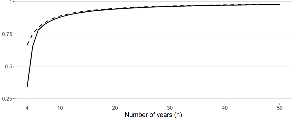
Figure 2: Rescaling factors (15) ( solid line ) and asymptotic upper bound (n - 2)/(n - 1) ( dashed line ).
