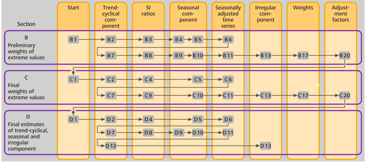
Figure 1: Basic workflow of the X-11 seasonal adjustment method as implemented in JDemetra+.
