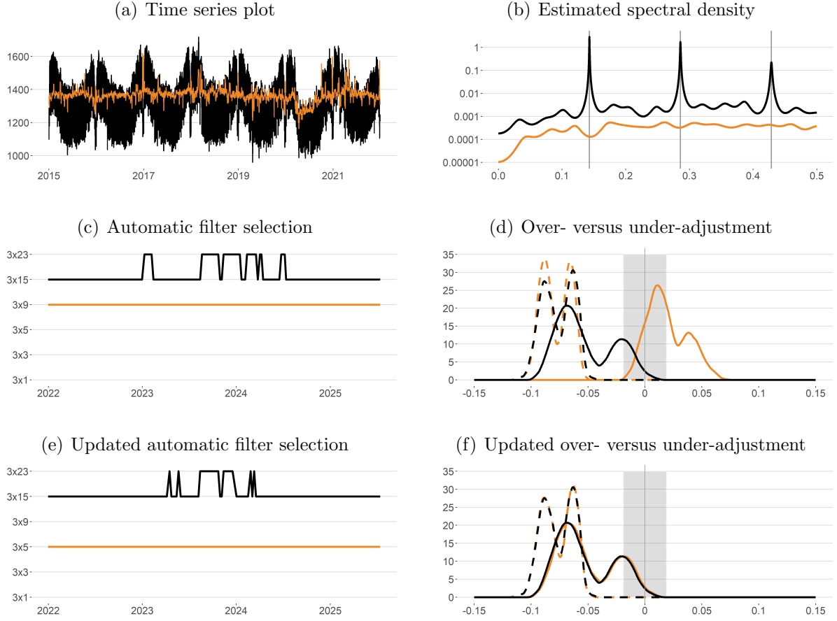
Figure 5: Results for daily electricity consumption. Panel (a) shows the unadjusted data in GWh units ( black line , W01 2022 vintage) and the seasonally adjusted data obtained via the [QR3, QR1] rule when extracting the day-of-the-week (DOW) pattern ( orange line ). Panel (b) shows the AR(30) estimate for the spectral density of the two differenced logged series (in decibels, abscissa in units of cycles per time). Grey verticals mark the three day-of-the-week frequencies. Panels (c) and (e) show the 3 \times k seasonal filters picked by the [QR3, QR1] rule when extracting the DOW ( orange line ) and day-of-the-year (DOY) patterns over the W01 2022 through W29 2025 vintages; the difference between the two scenarios is whether (e) or not (c) the DOY dynamics in (21) are recognised when selecting the seasonal filter for DOW extraction. Panels (d) and (f) show corresponding Epanechnikov kernel density estimates for \hat{\rho}_7 ( solid lines ) and \hat{\rho}_{365} ( dashed lines ) obtained from the differenced logged seasonally adjusted data using the 3 \times k seasonal filters picked by the [QR3, QR1] rule ( orange lines ) and the X-11 default filters ( black lines ) for DOW extraction. The shaded area marks \pm 1 Bartlett approximation to the large-lag standard error of \hat{\rho}_7 .
