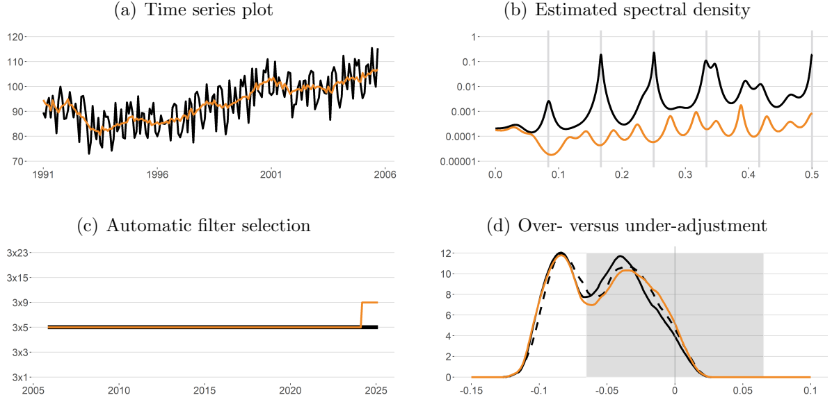
Figure 4: Results for monthly industrial production. Panel (a) shows the unadjusted data ( black line , 2000 = 100, November 2005 vintage) and the seasonally adjusted data obtained via the [QR3, QR1] rule ( orange line ). Panel (b) shows the AR(30) estimate for the spectral density of the two differenced logged series (in decibels, abscissa in units of cycles per time). Grey verticals mark the six seasonal frequencies. Panel (c) shows the 3 \times k seasonal filters picked by the classical ( black line ) and [QR3, QR1] ( orange line ) rules over the November 2005 through February 2025 vintages. Panel (d) shows Epanechnikov kernel density estimates for \hat{\rho}_{12} obtained from the differenced logged seasonally adjusted data with ( solid black line ) and without ( dashed black line ) hard-coding the seasonal filter picked by the classical rule. The shaded area marks \pm 1 Bartlett approximation to the large-lag standard error of \hat{\rho}_{12} .
