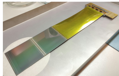
Figure 5: Module mock-up with two chained DSSDs.
