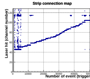
Figure 4: Response of the strips (numbering at y-axis) to the focused laser beam moving across the p-side strips as number of events (x-axis) grows up.
