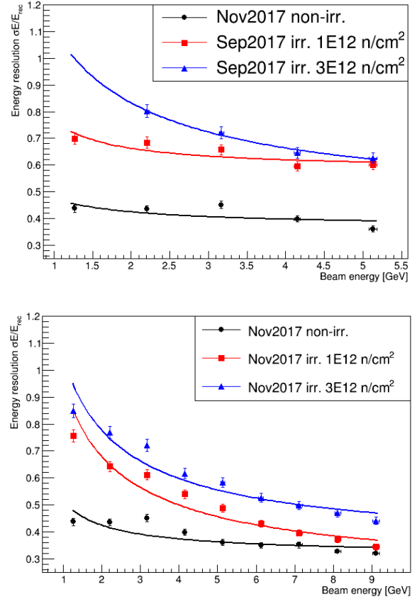
Figure 2: (top) Relative energy resolution measured for the proton beam energy scan from 1.3 up to 5.1 GeV at the T10 CERN beamline. (bottom) Relative energy resolution measured for the proton beam momentum scan from 1.3 up to 9.1 GeV at the T9 CERN beamline. Half of CBM PSD module was equipped with Hamamatsu SiPMs irradiated by neutrons with fluences of 1 \times 10^{12} and 3 \times 10^{12} n/cm 2 .
