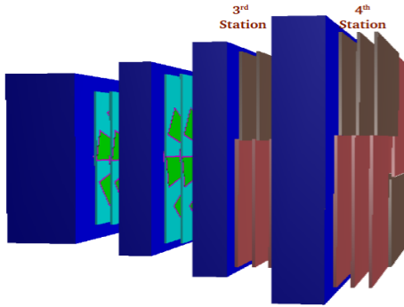
Figure 1: MUCH geometry with RPCs in the 3 rd & 4 th station.
