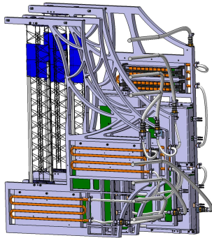
Figure 1: mSTS detector assembly.
