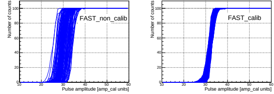
Figure 2: S-curves from the fast discriminator of all channels in the STS-XYTER v2 before and after calibration.
