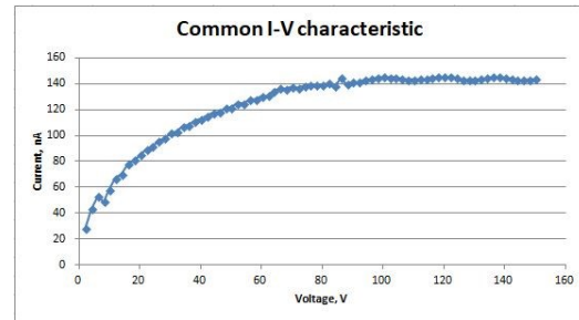
Figure 2: Common IV characteristic.
