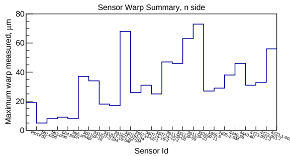
Figure 4: Summary of measured warp looking onto the n-sides of the prototype sensors available.
