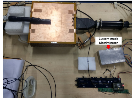
Figure 3: Cosmic Ray Test Setup of the RPC with PADI as FEE
