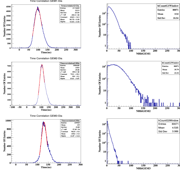
Figure 3: Top: Time difference between GEM1 and diamond (left) and average number of hit per event for GEM1(right). Middle: Same for GEM2. Bottom: Same for GEM3
