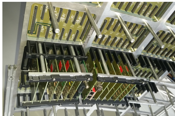
Figure 2: Close view of the prototype back side showing the fixation scheme for the front end modules.
