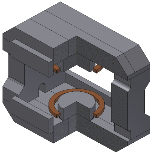
Figure 1: BINP design of the CBM magnet.
