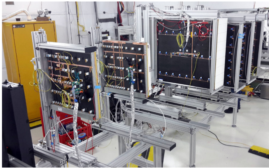
Figure 1: Experimental setup at DESY. Beam table and mounted TRD MWPCs with SPADIC 2.0 front-end boards.
