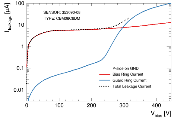
Figure 2: Bulk and surface currents of a 6 \times 6 \text{ cm}^2 CiS sensor as a function of reverse bias voltage.
