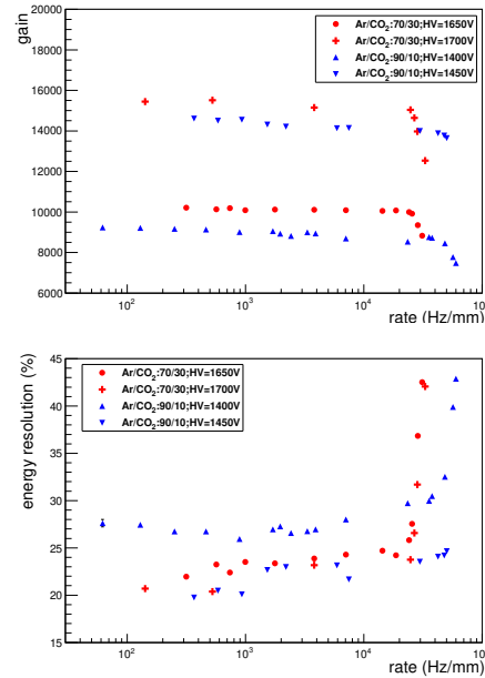
Figure 2: Gain and energy resolution as a function of rate for both Ar/CO 2 70/30 and 90/10 mixtures.
