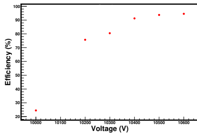
Figure 5: Efficiency as a function of applied high voltage
