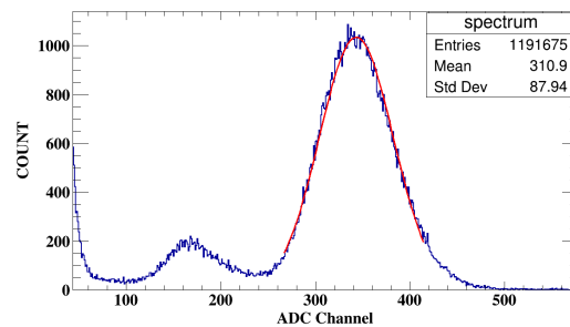
Figure 2: Typical Fe^{55} spectrum
