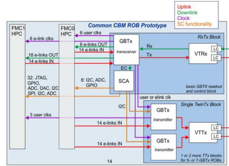
Figure 1: Functional diagram of the CROB.
