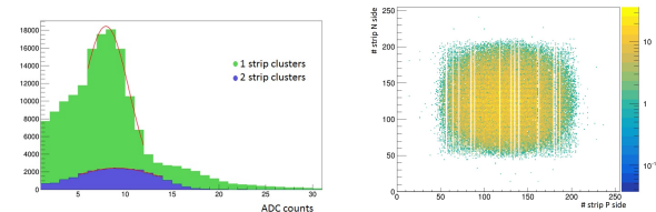
Figure 3: ^{241}\text{Am} gamma spectrum (left). Hit map of baby sensor with ^{241}\text{Am} gamma source (right).
