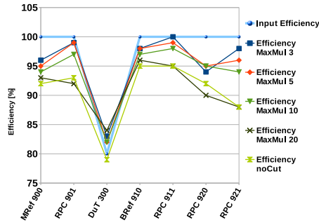
Figure 1: Efficiency results from the detector analysis chain for different maximum single counter hit multiplicities compared to simulation input
