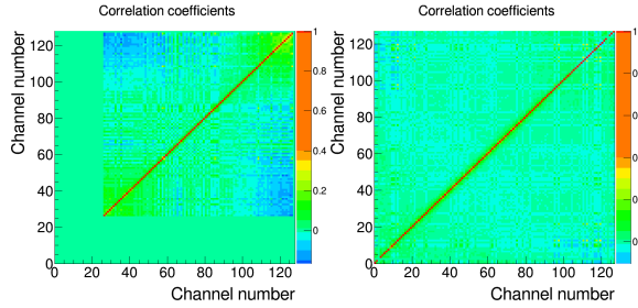
Figure 1: Correlation pattern for Module 1 (left panel) and Module 2 (right panel) between all channel pairs.
