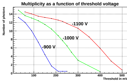
Figure 1: Hit multiplicity as a function of threshold. Different colors represent different MAPMT operating voltages.
