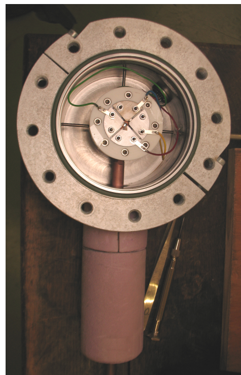
Figure 2: Photo of manufactured cell with beam monitoring metal plates arranged around titanium window.
