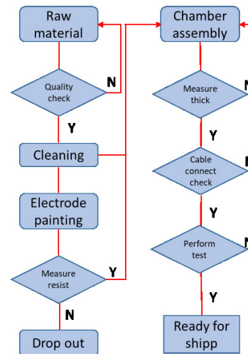
Figure 3: QC&QA production diagram.
