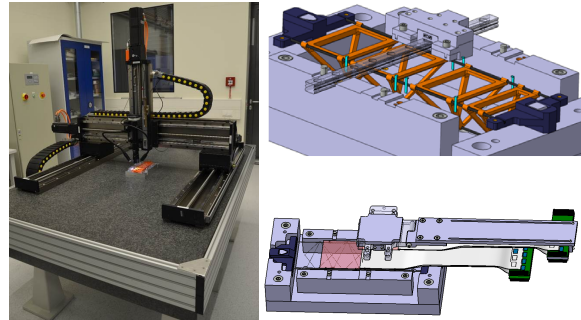
Figure 1: Movable camera system for inspecting assembled ladders (left); Positioning tool to holding two L-legs and a module during assembly (right).
