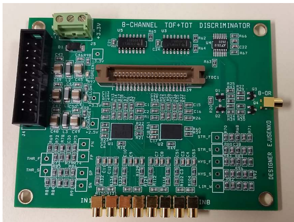
Figure 6: Photo of ToT 8 channels board.
