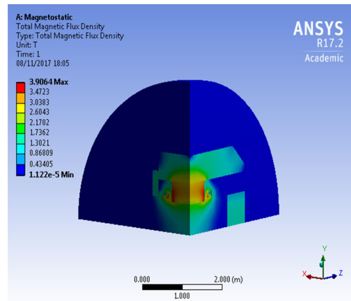
Figure 3: Total magnetic flux density.
