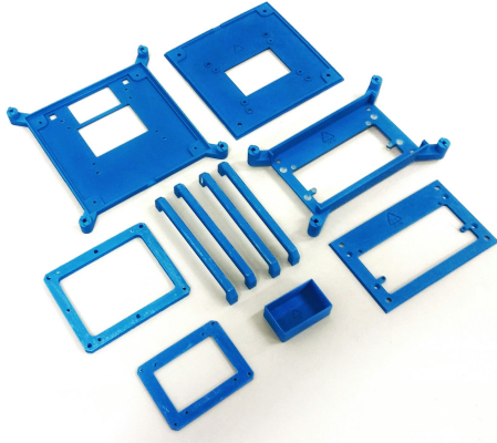
Figure 1: The 3D printed elements of the module support structure before assembly of the S^2M02 module.
