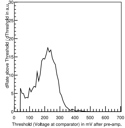
Figure 2: Differentiated statistical signal amplitude distribution. Derivation via five point stencil of measured rates, shown in figure 1.
