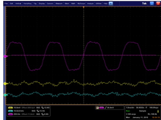
Figure 2: Crosstalk between one link carrying a 400 MHz LVDS signal and the neighbouring traces.
