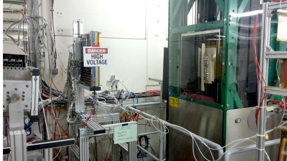
Figure 1: 2012-style TRD MWPC prototype installed in the downstream field of the GIF irradiator.
