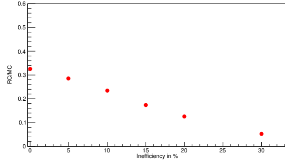
Figure 1: Variation of the single track reconstruction efficiency with detector in-efficiency (see text for more details).
