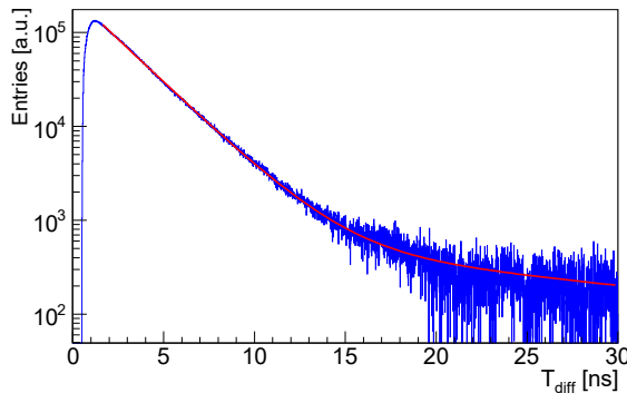
Figure 4: Blue: Difference between T_{\text{diff}} distributions for data with WLS coated and uncoated MAPMTs for a threshold of 80 mV. Red: Fit of the data with two exponential functions in a range between 1.5 ns and 40 ns.
