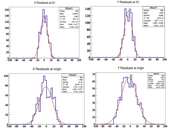
Figure 7: Residuals in X and Y at GEM1 plane(up) and Residuals in X and Y at diamond plane (down)
