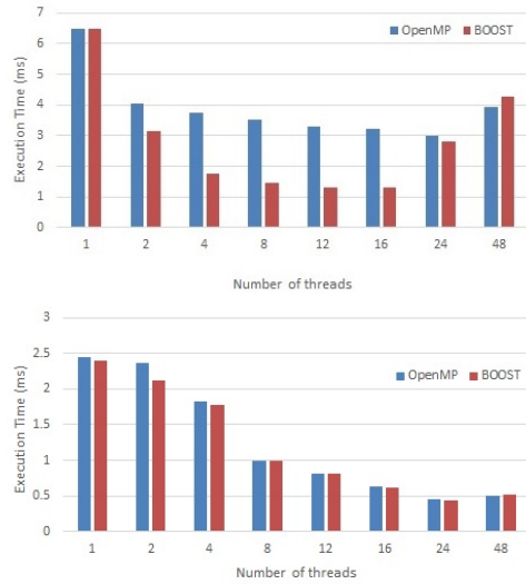
Figure 1: Execution time comparison for cluster finding (upper) and hit finding (lower) for a single event using the OpenMP and BOOST parallel paradigms
