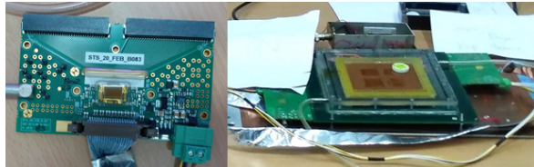
Figure 1: FEB-B MUCH-XYTER board in the left picture. Right picture shows ^{90}\text{Sr} test setup of MUCH-XYTER coupled with 10 cms X 10cms GEM detector at VECC
