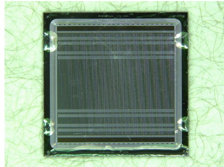
Figure 1: Baby sensor with glue applied at the guard rings where L-legs are attached for mounting on the ladder.
