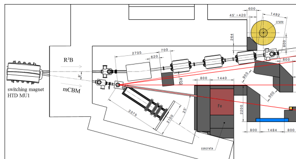
Figure 5: The modified mCBM cave (HTD) at the SIS18 facility of GSI/FAIR (as of August 31, 2017).
