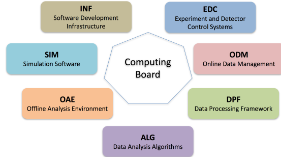
Figure 4: CBM computing project structure. Acronyms: EDC - Experiment and Detector Control System, ODM - Online Data Management, DPF - Data Processing Framework, ALG - data Analysis aLgorithms, OAE - Offline Analysis Environment, SIM - SIMulation software, INF - INFrastructure
