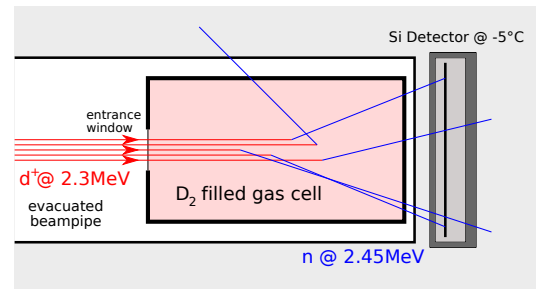
Figure 1: Schematic view of the cryogenic source.
