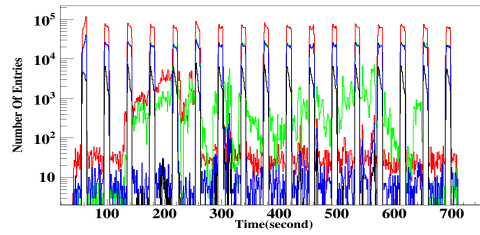
Figure 2: Spill structure seen for three different GEM plane and diamond detector
