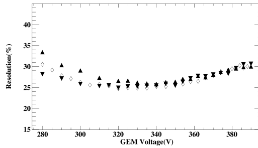
Figure 7: Variation of energy resolution with GEM voltage
