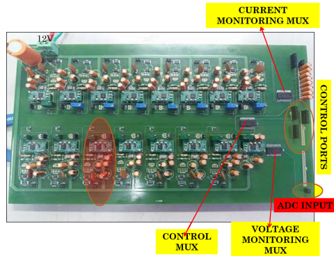
Figure 1: LVDB prototype
