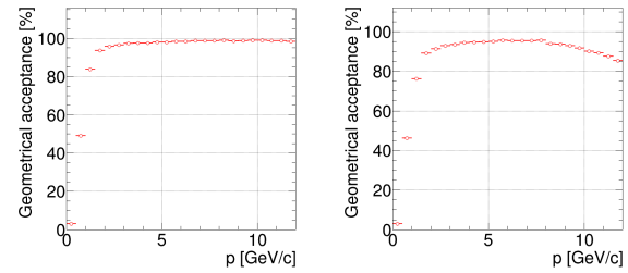
Figure 2: Geometrical acceptance for the rich_v18a_1e (left) and rich_v18a_3e (right) geometries
