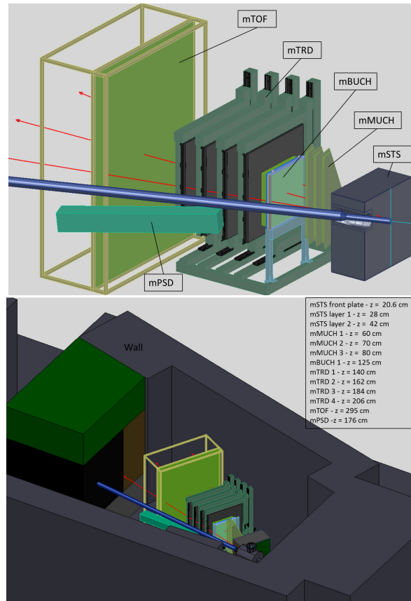
Figure 2: The mCBM set-up (top) and its positioning inside the HTD cave (bottom).
