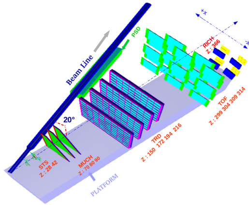
Figure 1: Schematic layout of the mCBM test-setup.
