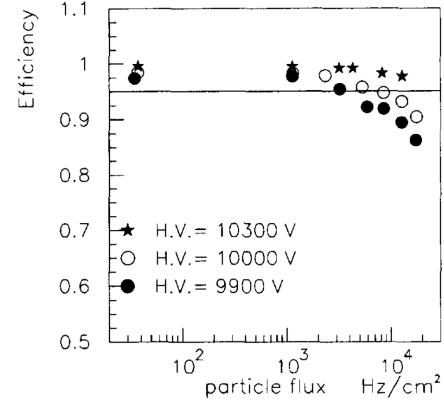
Figure 2: Efficiency of low resistivity RPC operating in avalanche mode as a function of particle flux for 3 different high voltage.[2]
