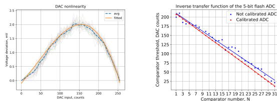
Figure 1: Non-linearity of DAC for test pulser (left); Correction of ADC (right).
