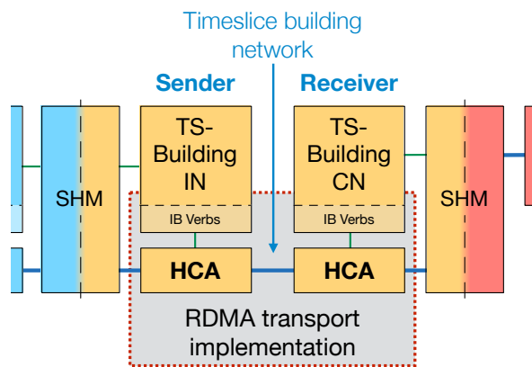
Figure 1: The data transport software is divided into modules, allowing the RDMA transport to be exchanged by a different implementation.
