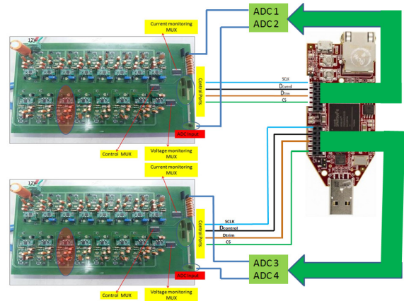
Figure 6: Full fledge control for two LVDB boards.
