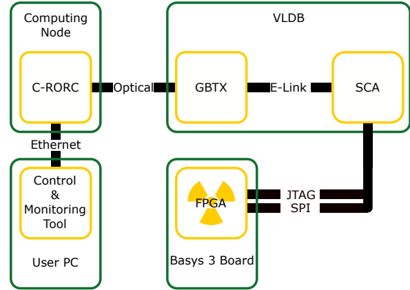
Figure 1: Schematic setup of the FPGA configuration and management setup. The interpretation and control of ongoing events is performed in the Control and Monitoring Tool on the User PC. The necessary Files (i.e. FPGA bitfile and single configuration frames) are held locally in the computing node.
