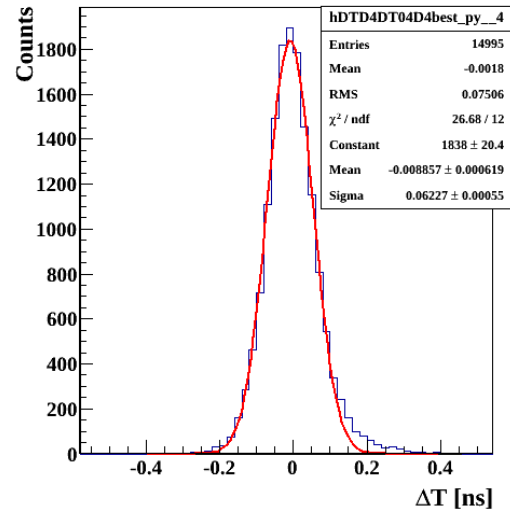
Figure 2: Time difference distribution between DUT and RPCref.
