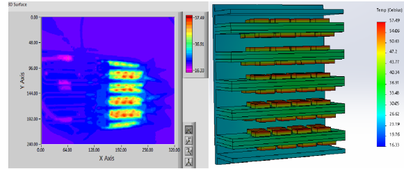
Figure 2: Comparison of experiment (IR camera) and simulation.
