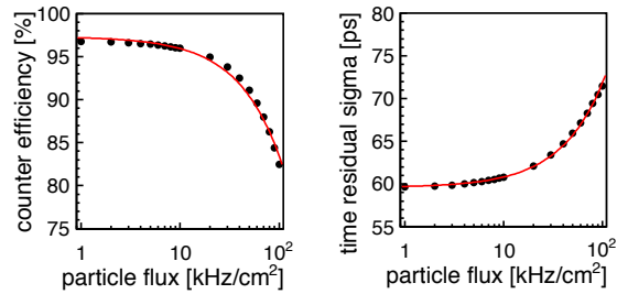
Figure 1: Average counter efficiency decline (left plot) and worsening of the time resolution (right plot) both as functions of an incident particle flux uniformly illuminating a surface spot of 1 \text{ cm}^2 on a 900 \text{ cm}^2 MRPC for 30 s. The lines correspond to linear fits to the simulated data.
