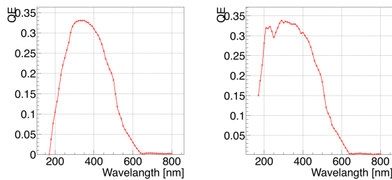
Figure 1: Quantum efficiency measurements in dependence on the photon wavelength. Left: H12700 MAPMT (default version in cbmroot ). Right: H12700 MAPMT covered with wavelength shifter film from p-terphenyl (WLS).
