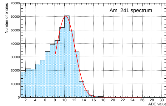
Figure 2: 241 Am spectrum measured with a silicon strip sensor and readout in a channel of the STS-XYTER v2
