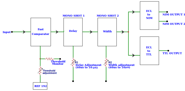
Figure 4: Functional Block Diagram of the Custom-made Discriminator
