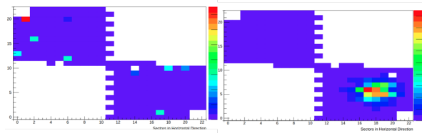
Figure 2: DAQ output of the GEM chamber attached to MUCH-XYTER. Left 2D plot is without source while right 2D plot is with ^{90}\text{Sr} source spot
