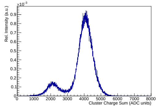
Figure 3: ^{55}\text{Fe} spectrum resulting from single event selection.
