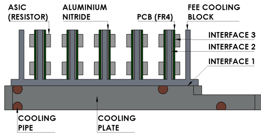
Figure 1: Experimental setup with thermal interfaces.
