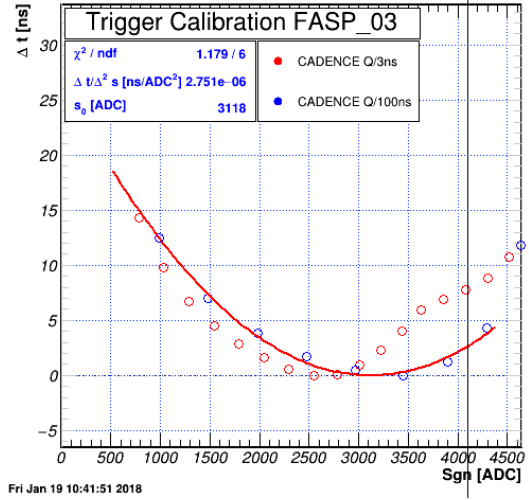
Figure 5: Latency of the FASP ASIC based on CADENCE™ simulations.
