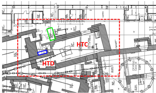
Figure 1: Experimental hall at SIS18: the area inside the red box are the caves HTD (mCBM) and HTC (R 3 B experiment).
