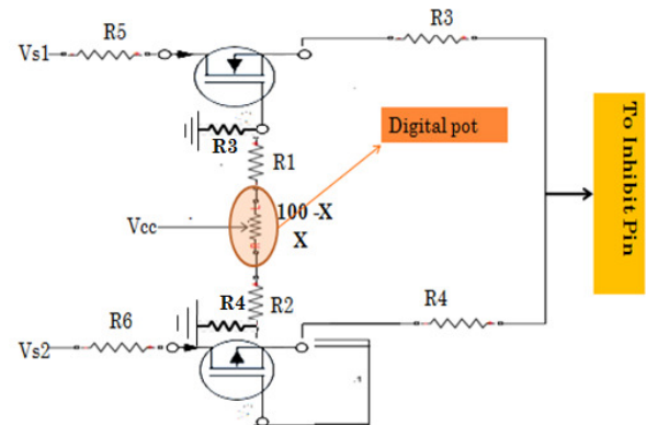
Figure 3: Schematic of hard on and stable off circuit
