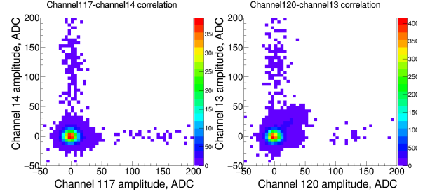
Figure 2: Typical correlation pattern for pairs of channels with low correlation \eta = -0.006 (left panel) and with medium correlation \eta = -0.33 (right panel) observed for Module 2.
