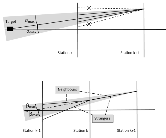
Figure 1: Top: segment set formation; bottom: segment binding procedure
