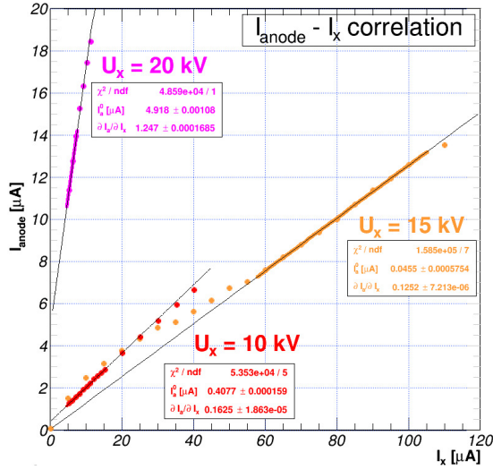
Figure 3: TRD anode wire ( I_{anode} ) as function of x-rays tube current ( I_x ) for 3 different x-rays spectra selected by the tube voltage U_x of 10, 15 and 20 kV. Linear fits are added to show the relation between the two observables.
