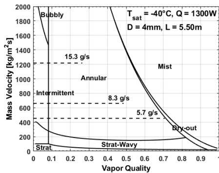
Figure 4: Flow pattern map for case #1 of Table 2.
