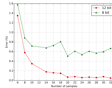
Figure 1: Accuracy of the online reconstructed total cluster charge, determined by comparing the results of the online and the offline cluster finder as a function of the numbers of signal samples. The values represent a charge calculation resolution of 12 bit and 8 bit, respectively.
