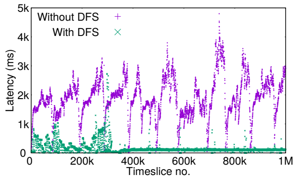
Figure 2: Latency between first and last contribution of timeslice
