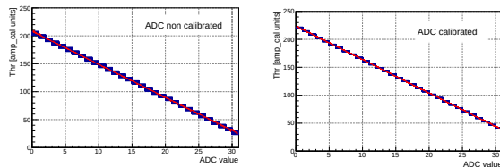
Figure 1: ADC transfer function for all the cahnnels in the STS-XYTER v2 before and after calibration.
