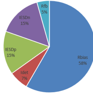
Figure 1: Components of the current noise i_n^2 .
