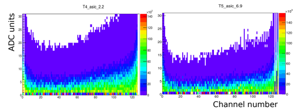
Figure 3: Noise performance of two recently assembled modules (n-side, 0 V bias voltage).
