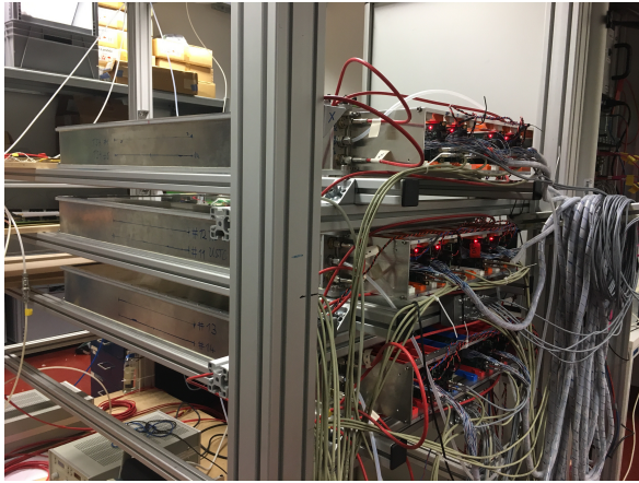
Figure 2: Photography of the Heidelberg cosmic setup. Three modules containing 2 counters each are placed on top of each other so that in total 6 counters can be tested simultaneously.
