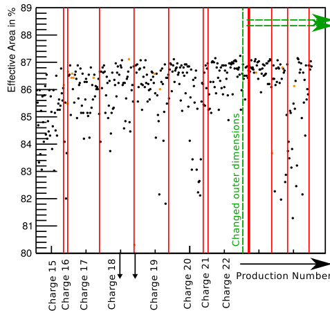
Figure 1: Effective area in percent. Only the last 400 measured MAPMTs are shown. The arrows to the bottom of the plot illustrate MAPMTs having an effective area lower than 80%. The MAPMTs measured after the green dashed line have smaller outer dimensions. The red vertical lines mark different delivery charges. The orange dots and arrows indicate that the measured MAPMT was supplied with a voltage of -1100 V.
