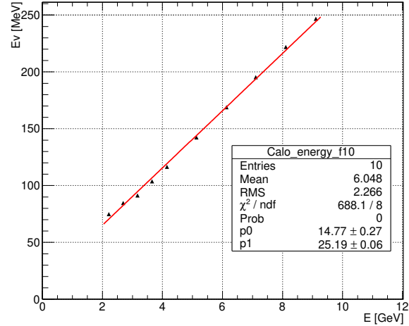
Figure 4: Supermodule energy as a function of the proton beam energies.
