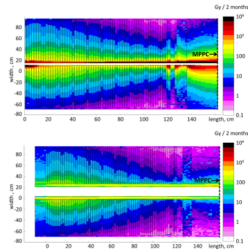
Figure 1: The ionizing energy loss at 4 AGeV for PSD with beam hole: 6 cm (upper picture) and 20 \times 20\ \text{cm}^2 (bottom picture) for horizontal cut.
