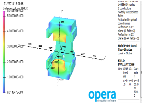
Figure 6: Magnetic field saturation picture.
