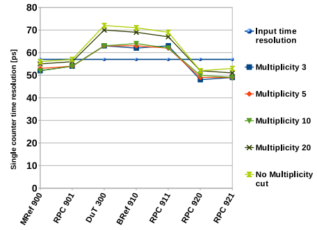
Figure 2: Time resolution results from the detector analysis chain for different maximum multiplicities compared to simulation input
