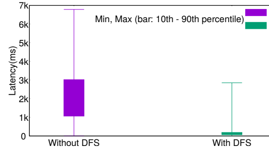
Figure 3: 10th-90th percentile of latency to receive timeslices
