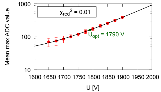
Figure 2: Mean maximum ADC value as a function of the anode voltage U_A , fit by ADC(U) = a \cdot \exp(b \cdot U)
