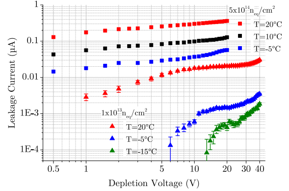
Figure 1: Leakage currents as function of the depletion voltage observed with PIPPER-2, with different operation temperatures and two non-ionizing radiation doses.
