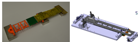
Figure 3: A non-function module mounted on a ladder (left); the assembly tool for the mSTS ladders (right).
