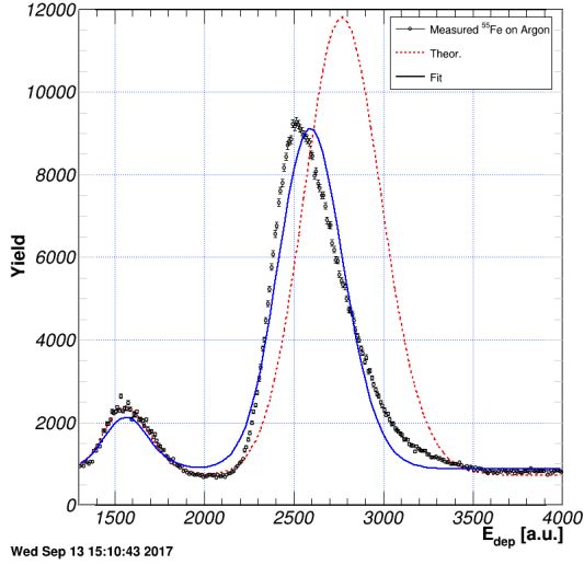
Figure 3: Gas gain calibration of the FASP ASIC based on ^{55}\text{Fe} measurements and CADENCE™ simulations.
