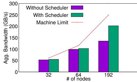
Figure 4: Aggregated bandwidth with/out DFS
