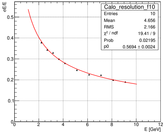
Figure 3: Energy resolution of the PSD supermodule for protons as a function of beam energy.
