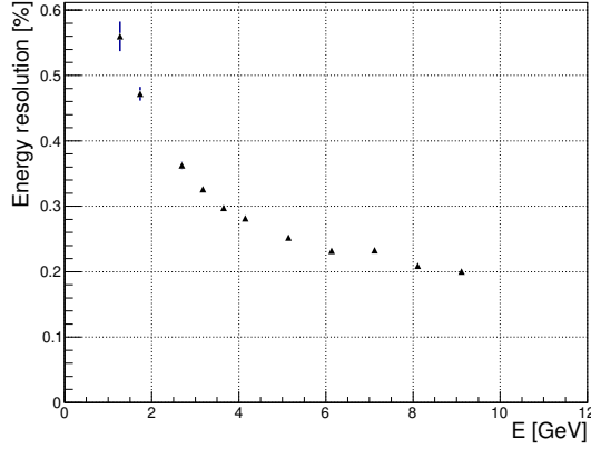
Figure 2: Energy resolution of mPSD response measured at T9/T10 beam lines at CERN.
