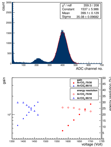
Figure 1: (Top) Energy spectrum of the straw tube detector with the Gaussian fitting curve (red line) to the 5.9 keV peak. (Bottom) The Gain and the energy resolution vs. voltage.
