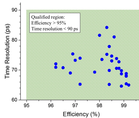
Figure 7: The analyzed efficiency and time resolution of the counters tested with cosmic ray. All of them meet the requirement of over 95% efficiency and below 90 ps time resolution (marked by the green dashed region).
