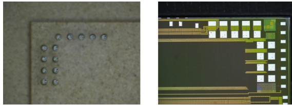
Figure 2: Close-up view of the Pogo Pins and mirrored contact area on the STS-XYTER ASIC
