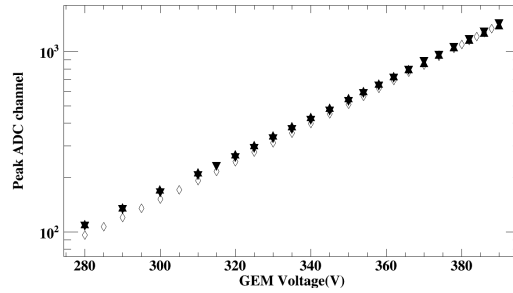
Figure 6: Variation of peak ADC channel with GEM voltage
