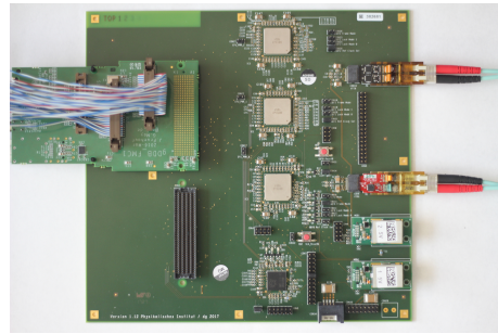
Figure 2: The CBM CROB prototype board.
