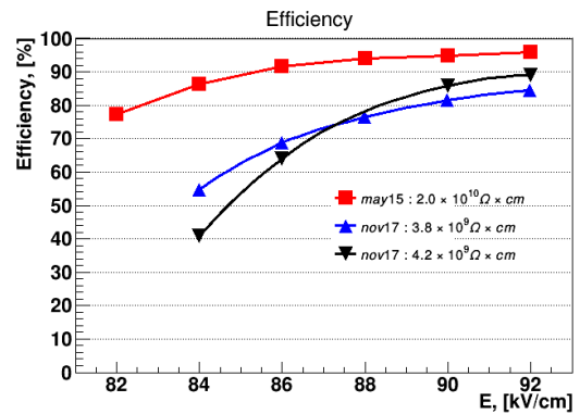
Figure 3: Comparison of the high voltage scans performed with different readout: squares - MAXIM3760+CAEN TDC, triangles - PADI+VFTX TDC.
