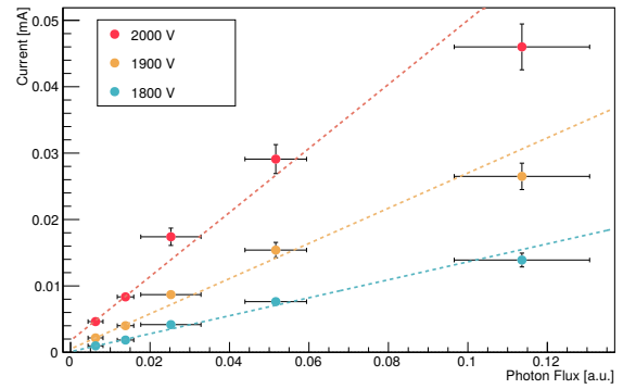
Figure 2: Measured anode currents for three voltage levels wrt. the relative photon flux. Lines: linear fits to the data.
