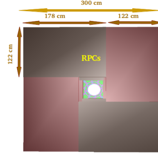
Figure 2: Rectangular shaped RPC modules for 3 rd station.
