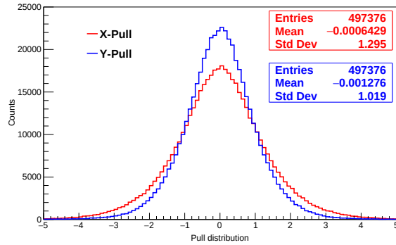
Figure 2: X-Y directional pull distribution
