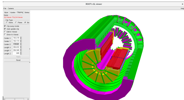
Figure 6: eTOF geometry included in the STAR simulation framework.
