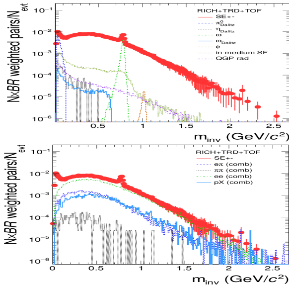
Figure 1: Invariant mass distribution for different unlike-sign pairs identified as electrons for central (10 %) Au+Au collisions at 8 AGeV (red points), together with various signal channels (upper panel) and the combinatorial background contributions (lower panel). All contributions are weighted with their expected yield and branching ratio.
