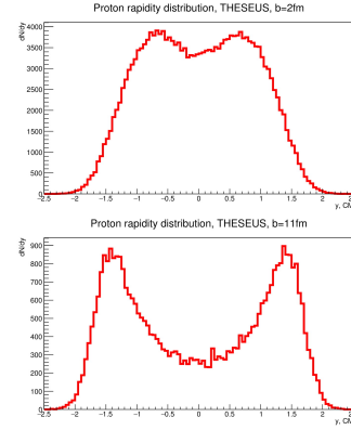
Figure 2: Proton rapidity distributions for THESEUS events at 10 AGeV and impact parameters 2fm and 11fm.
