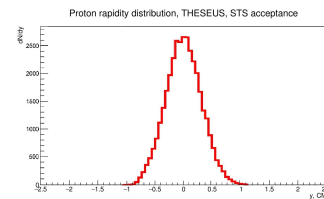
Figure 3: Proton rapidity distribution for THESEUS events at 10 AGeV, b = 2 fm and STS simulation and reconstruction.
