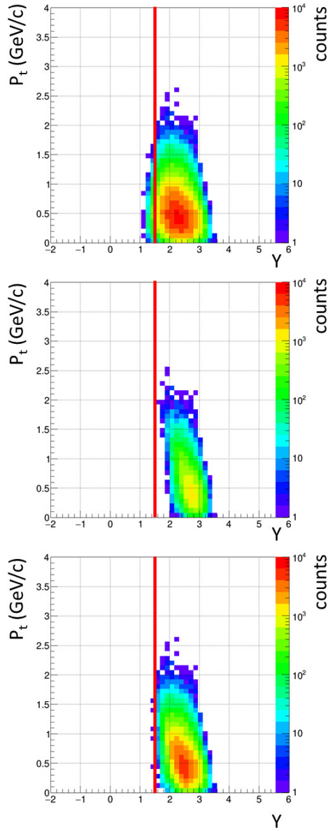
Figure 2: Acceptance for reconstructed muon pairs as function of transverse momentum and rapidity. Upper panel: muon pairs from all muon track candidates. Center panel: muon pairs from long tracks traversing 1 m iron absorber. Lower panel: muon pairs from short and long tracks (see text). The red lines refer to mid-rapidity for 8 AGeV.
