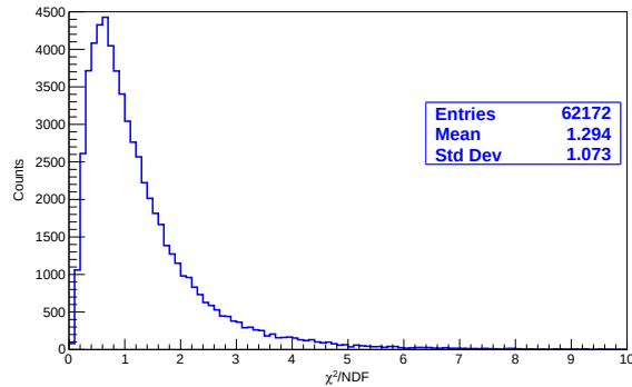
Figure 3: \chi^2/\text{NDF}
