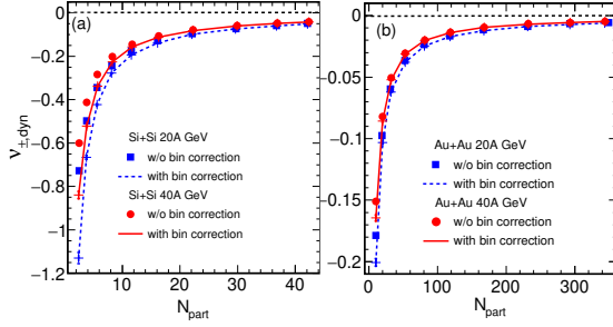
Figure 2: \nu_{\pm,\text{dyn}} calculated without (w/o) and with the finite width multiplicity bin correction, are plotted against N_{\text{part}} for Si+Si and Au+Au collisions at 20A and 40A GeV
