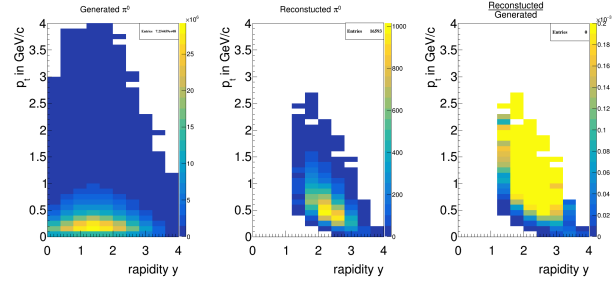
Figure 1: Phase-space coverage of all generated \pi^0 on the left plot, all reconstructed \pi^0 via conversion method on the middle plot, together with their ratio on the right plot.
