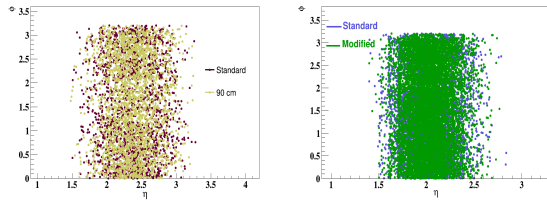
Figure 5: \eta - \phi of reconstructed \omega at 8 AGeV (left) and for reconstructed J/\psi at 25 AGeV (right).
