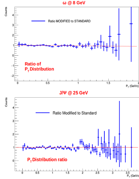
Figure 6: p_T wise efficiency ratio of modified to standard setup of \omega at 8 AGeV (top) and for J/\psi at 25 AGeV (bottom).
