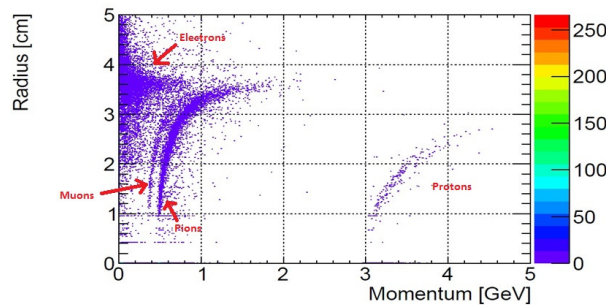
Figure 5: RICH ring radius versus the particle momentum for 100.000 events in mCBM (1.24 GeV Au + Au collisions)
