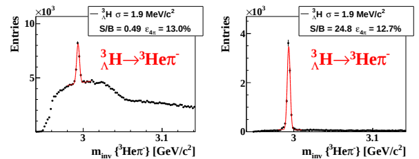
Figure 2: ^3_\Lambda\text{H} reconstruction involving only TOF (left panel) and with an additional PID from STS (right panel). 5 \times 10^6 central Au+Au collisions at 10 A GeV were simulated.
