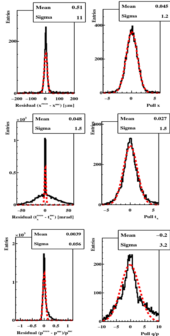
Figure 2: Distributions of residuals (left) and pulls (right) for the x , t_x and q/p track parameters obtained with Kalman Filter track fit at the last hit position in the combined STS+MUCH system. The dashed red curve reflects a Gaussian fit to the distribution, the parameters of which are shown in the panels.
