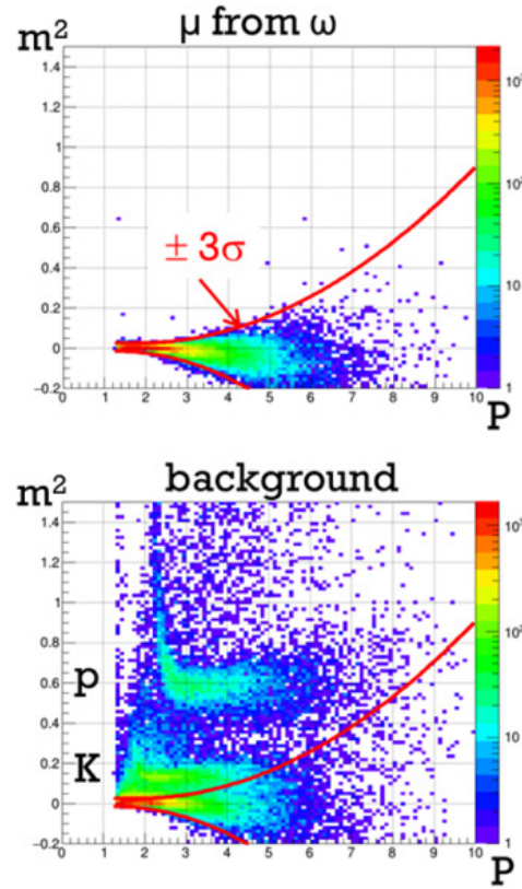
Figure 1: Squared mass distributions versus momentum of muons from omega meson decays (upper panel) and for protons, kaons and pions (lower panel) using ToF measurements. The red lines represent a 3 sigma Gauss fit for the selection of muon candidates by ToF.
