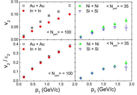
Figure 3: p_T dependence of v_2 (upper panel) and v_2/\varepsilon_2 (lower panel) of charged hadrons for different colliding systems at E_{\text{lab}} = 30A GeV.
