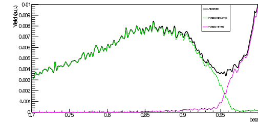
Figure 6: \beta distribution for all particles in mCBM in the mTOF and mRICH acceptance: Green no ring seen in mRICH, purple; ring seen in mRICH.
