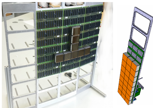
Figure 1: The CBM RICH photon detector prototype front side, consisting of 4 aluminum frames partly equipped with backplanes and PMTs; and a schematic drawing of a single frame element.
