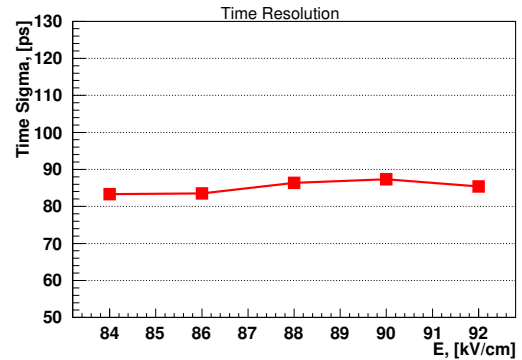
Figure 5: Time resolution of the cell 3 (bulk resistivity is 3.8 \cdot 10^9 \Omega \cdot \text{cm} ) as function of the applied electric field.
