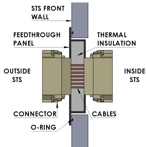
Figure 3: Structure of the feed-through panel.
