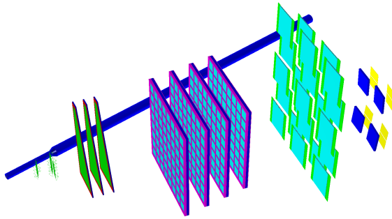
Figure 1: The mCBM setup, consisting (from left to right) of two stations of mSTS, three layers of mMUCH, four stations of mTRD, mTOF and mRICH. All detectors are arranged on one side of the beam. There is no magnetic field.
