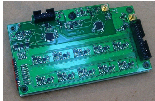
Figure 3: A ten channel FEE board with differential outputs.
