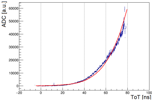
Figure 8: The response curve of ToT board. The red line is a second order polynomial fit.
