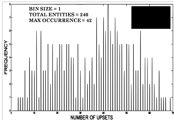
Figure 1: Occurrence of SEUs with 2 min refresh rate
