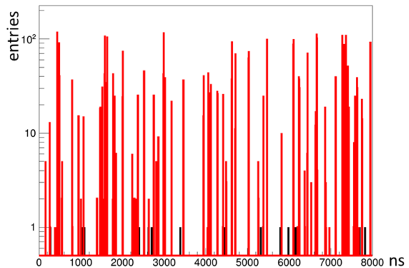
Figure 2: Time distribution of reconstructed STS tracks for a Au beam intensity of 10^9 ions/s at 8 A GeV. The red histogram corresponds to minimum-bias UrQMD Au+Au events, the black histogram represents \delta -electrons produced by Au ions passing through the Au target.
