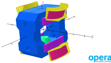
Figure 1: Magnet (blue) and shielding box (yellow) with photodetector (pink) implemented in the TOSCA simulations. (The appearance of the shielding boxes on both sides of the magnet is an artefact of symmetries used in the calculations.)
