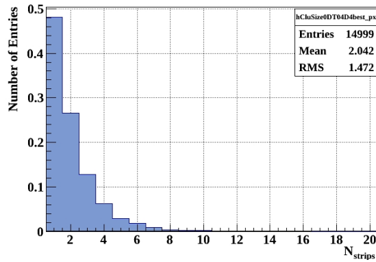
Figure 3: Cluster size distribution for 200 mV electronics threshold.
