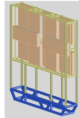
Figure 4: Space frame.
