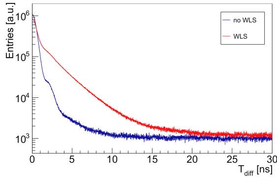
Figure 3: Distribution of T_{\text{diff}} for WLS coated (red) and uncoated (blue) MAPMTs in the RICH Testbox at a threshold of 80 mV, produced from cherenkov photons at a 1.25 GeV/c proton beam. The Diagrams are normalized to the same number of events.
