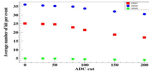
Figure 5: Variation of average number of hit per event with ADC cut
