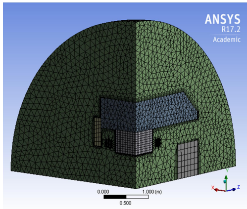
Figure 2: Mesh of 1/8 magnet model.
