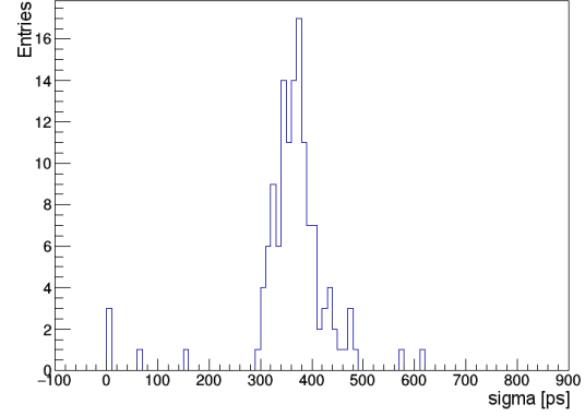
Figure 2: Distribution of time precision from 144 channels (Threshold: 80 mV).
