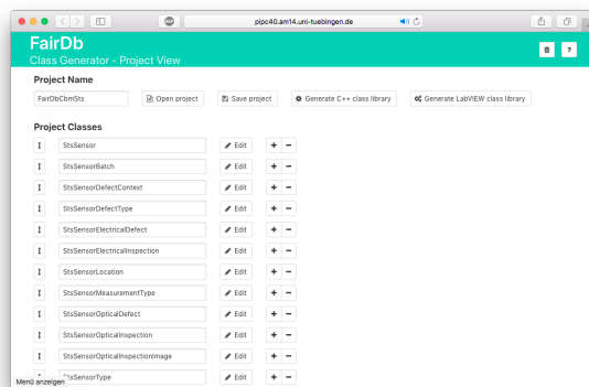
Figure 1: Graphical user interface to define the database classes organized in projects.
