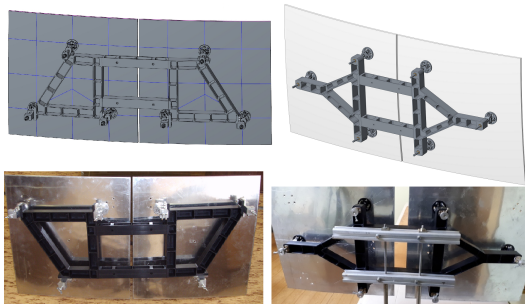
Figure 1: Previous (left) and new (right) design of the small frame. Top row: design models. Bottom row: photo of the produced frames with aluminum plates to imitate the mirror tiles.
