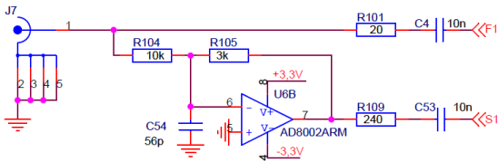
Figure 7: Schematic view of one channel of ToT board.
