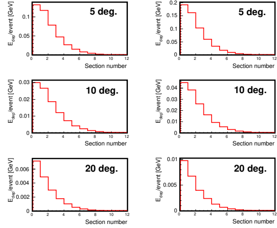
Figure 4: Energy deposition in mPSD sections for reactions Ag+Ag@1.65 AGeV (left column) and Au+Au@1.23 AGeV (right column) for different mPSD angle relative to the beam axis.
