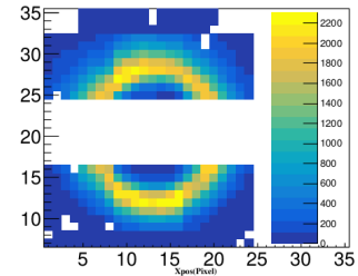
Figure 2: The proximity focusing setup with a 3 mm thick quartz glass radiator (left), and a typical integrated 2d hit map obtained with this setup.
