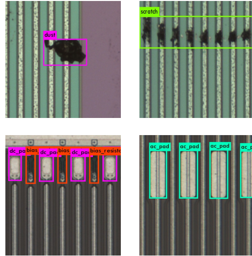
Figure 2: Detection of the defects (dust particle and scratch, top panels) and electrical elements (DC pads, bias resistors and AC pads, bottom panels) with neural network.
