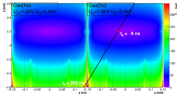
Figure 1: Track splitting in the TRD volume in the y - z plane according to amplification cells
