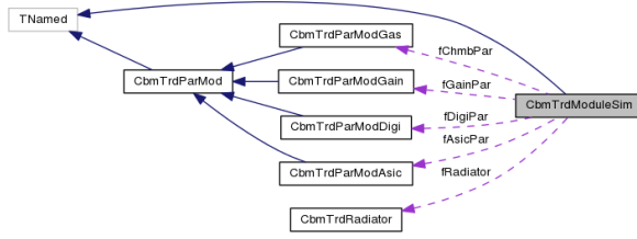
Figure 7: Collaboration map of the CbmTrdModuleSim class with calibration classes
