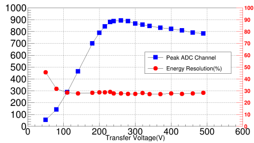
Figure 4: Variation of ADC and energy resolution with transfer voltage
