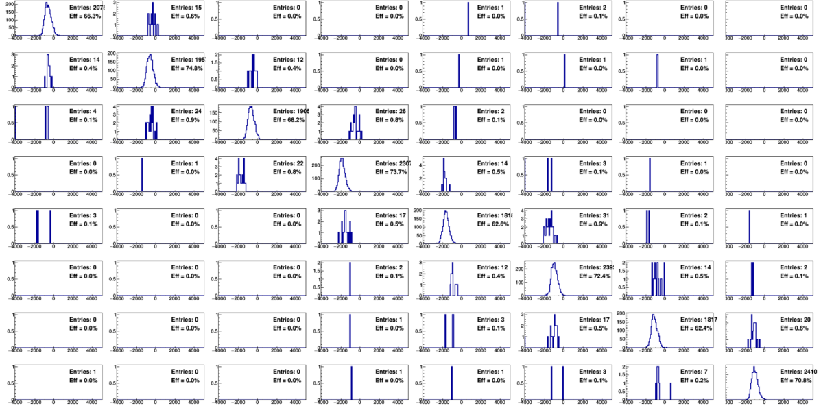
Figure 4: Cross-talk probability measurements. Time spectra of the signals passing the narrow trigger are shown for all cells of the minimodule. The number of entries and registration efficiency are shown for every cell. The ratio of this values to the corresponding values of the trigger cell defines the cross-talk probability.
