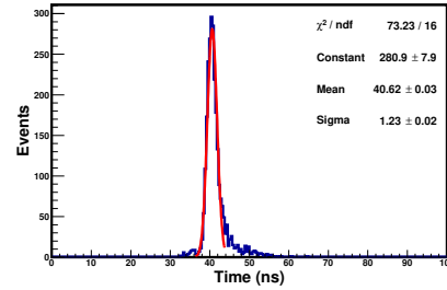
Figure 7: Raw timing spectra using a 12 bit TDC
