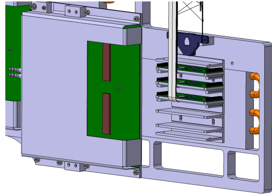
Figure 2: Front-End boards of the mSTS.
