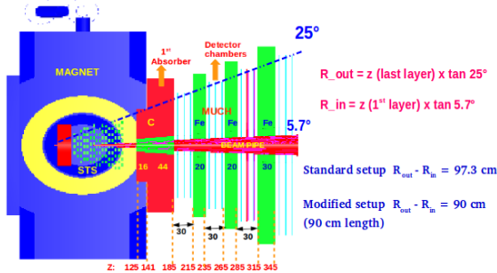
Figure 1: Sectional view of the CBM-MUCH geometry.
