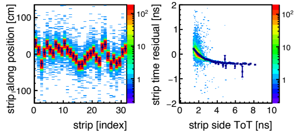
Figure 2: Signal position misalignment along the readout strips (left plot) and dependence of the signal time residual on the time over threshold (“time walk”; right plot) as introduced in the new digitization scheme.
