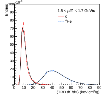
Figure 2: \langle dE/dx \rangle distributions for d and {}^4\text{He} , as reconstructed with the TRD, fitted with a modified Gaussian.
