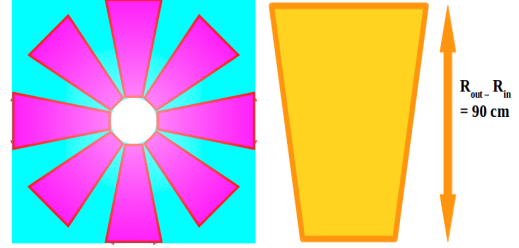
Figure 2: Arrangement of modules in the 1 st station. Read-out plane of a module has been shown separately.
