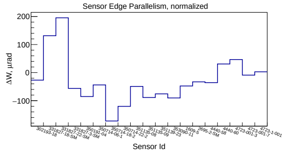
Figure 3: Summary of the parallelism measured for available prototype sensors. The values normalized to the edge length are expressed in micro radians.
