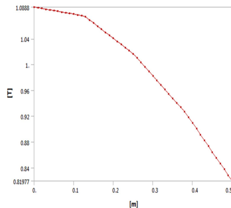
Figure 4: Magnetic field along the beam axis.
