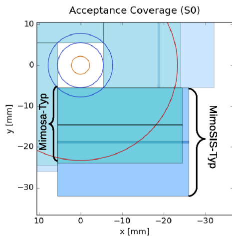
Figure 1: Comparing MIMOSA vs. MIMOSIS sensor layouts (2 adjacent sensors, station 0, front side) in one quadrant. Circles depict the geometrical acceptance.
