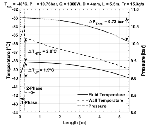
Figure 5: Temperature and pressure distribution along the cooling pipe.
