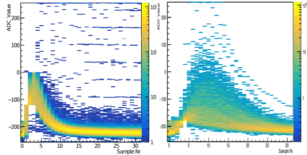
Figure 2: Overlaid signal shapes with SPADIC 1.0 (left) and SPADIC 2.0 (right) using the same set of analysis classes.
