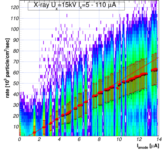
Figure 4: An overview of the rate performance of the TRD17 prototype in HCR x-rays environment as a function of the anode wire current. Average values as well as linear trending are added in red to illustrate current performance/limitations of the system.
