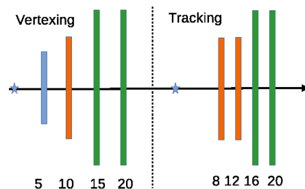
Figure 2: New MVD geometries with stations 0-3. Left: “Vertexing”, right: “Tracking” geometry. Colors depict the station layout, i.e. three different station layouts in total. Numbers indicate the distance to the target in cm.
