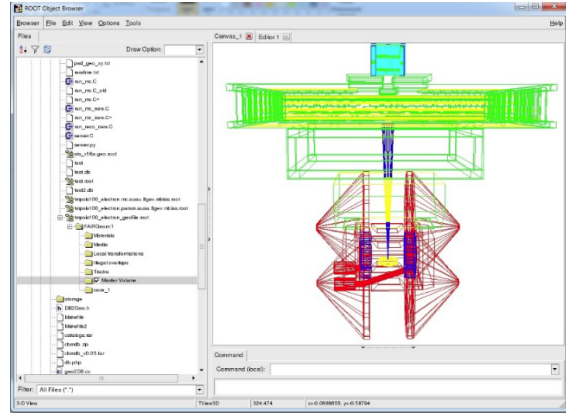
Figure 2: Example of executing the loadSetup macro - the “sis100_electron” setup loaded from the Geometry DB
