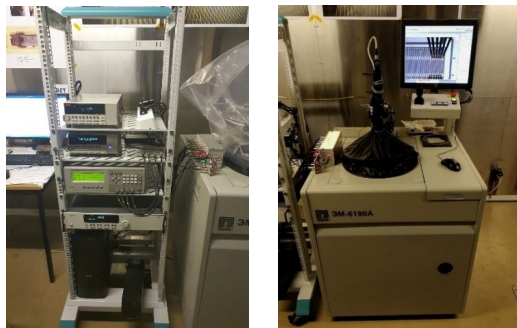
Figure 1: VB LHEP DSSD automatized test stand: rack with measuring electronics (left); automatic prober based on EM-6190A chip prober manufactured by PLANAR (right).
