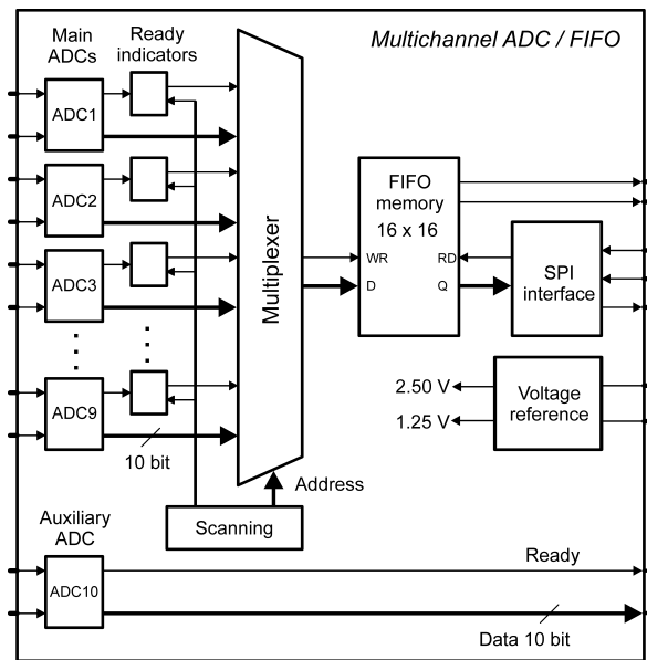
Figure 1: Architecture of multichannel ADC
