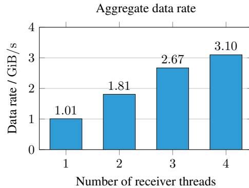
Figure 2: ZeroMQ Flesnet transport performance in a test setup with 8 FLIB links
