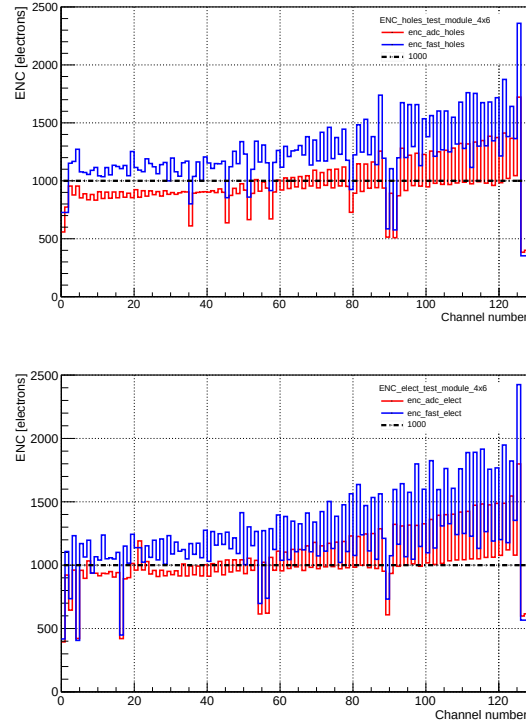
Figure 3: Noise level for holes and electrons measured for a 4.2 \times 6.2 cm 2 silicon sensor coupled to a 25 cm microcable and readout with the STS-XYTER v2 ASICs
