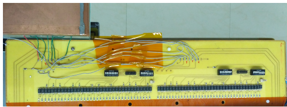
Figure 1: Section of drift chamber mounted with optocouplers and HV connections
