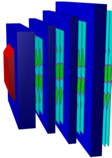
Figure 2: Schematic view of the SIS100B MUCH geometry
