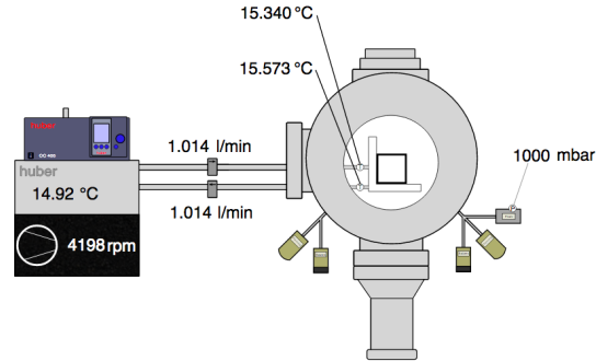
Figure 2: A graphical overview of the vacuum test bench of PRESTO
