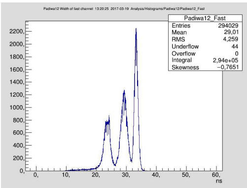
Figure 9: Signals of ToT measured with TRB3 board. From left to right: 5mV, 20mV, 40mV.
