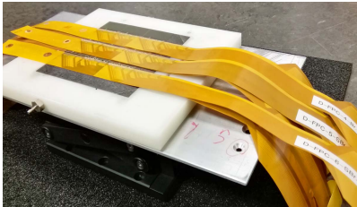
Figure 1: PRESTO front side equipped with nine M26 sensors, wire-bonded to dedicated low-mass flex cables.
