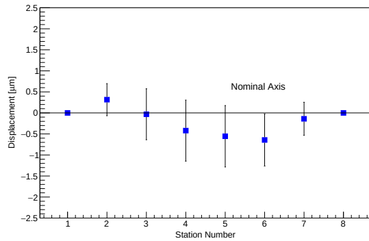
Figure 1: Station displacements after realignment.
