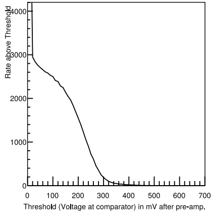
Figure 1: Measured rate above threshold for different thresholds. Measured in one channel of one DiRICH during constant illumination with single photons.
