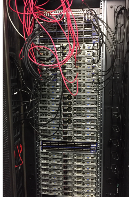
Figure 2: New part of the mFLES test cluster installed in rack 61 in the Green IT Cube data center at GSI. 12 of the 48 available nodes are cabled for first tests.
