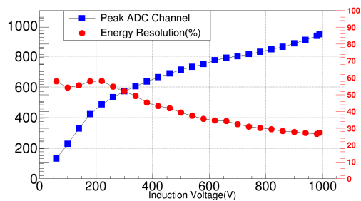
Figure 5: Variation of ADC and energy resolution with induction voltage
