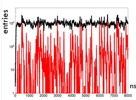
Figure 1: Time distribution of the digital signals from the STS for a Au beam intensity of 10^9 ions/s at 8 A GeV. The red histogram corresponds to minimum-bias UrQMD Au+Au events, the black histogram represents \delta -electrons produced by the Au ions passing through the Au target.
