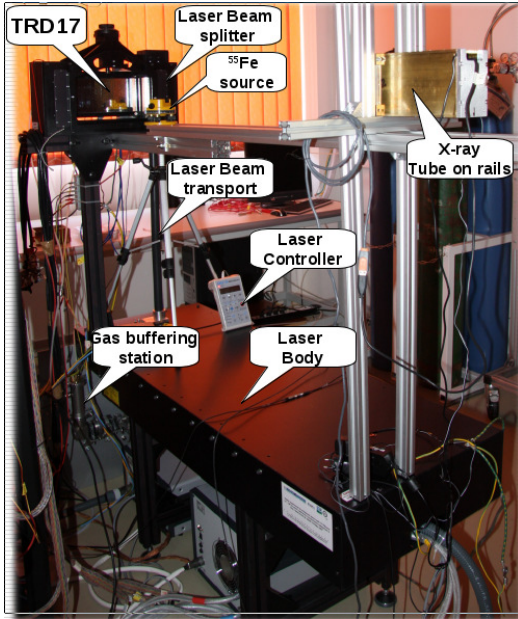
Figure 1: The TRD17 prototype mounted on its test stand to monitor system performance in HCR.
