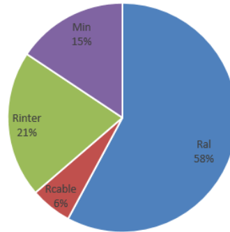
Figure 2: Components of the voltage noise v_{nw}^2 .
