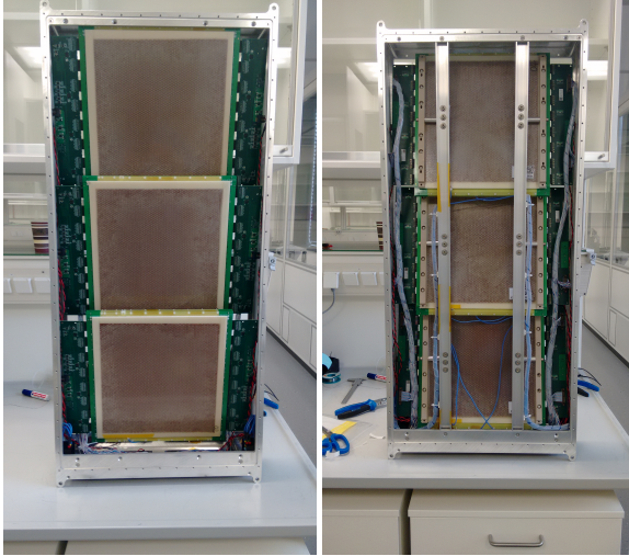
Figure 3: Open eTOF module - left: front side, right: back side.
