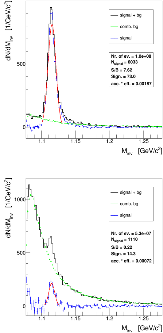
Figure 8: \Lambda -identification in minimum bias UrQMD events in Ni+Ni collisions at 1.93 AGeV (top) and in Au + Au at 1.24 AGeV (bottom). Invariant mass distributions are shown for (\pi^- p) pair combinations (combinatorics) within events (black line, signal + bg), for pair combinations from mixed events (green symbols, comb. bg) and for the resulting distribution after subtraction (blue symbols, signal). Statistics information is obtained from a Gaussian fit to the subtracted distribution (red line).
