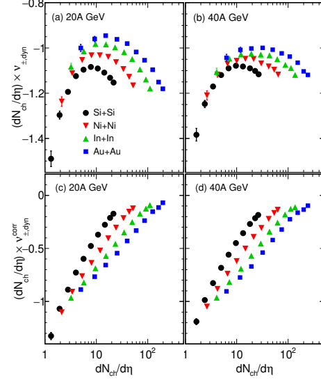
Figure 4: Dynamical net-charge fluctuations multiplied by dN_{\text{ch}}/d\eta|_{\eta=\eta_0} are plotted against dN_{\text{ch}}/d\eta|_{\eta=\eta_0} .
