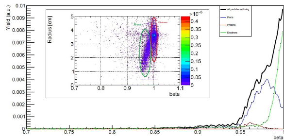
Figure 7: \beta distribution for all particles in mCBM leaving a signal in the ToF and producing a ring in the RICH: protons (red), pions (blue), electrons (green) Inner plot: RICH ring radius versus velocity \beta .
