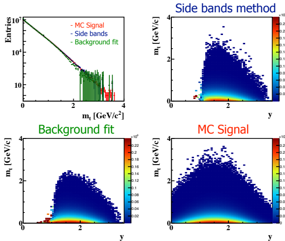
Figure 1: Efficiency corrected spectra of K_s^0 \rightarrow \pi^+\pi^- decay as a function of m_t and y - m_t obtained by the side bands and background fit methods in comparison with the simulated MC signal from 5M central AuAu UrQMD events at 10 AGeV.
