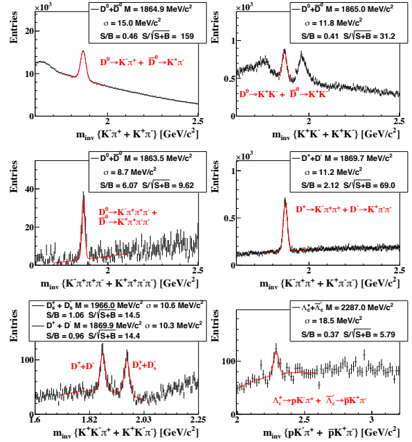
Figure 1: Invariant mass distributions of D -mesons and \Lambda_C reconstructed with the KF Particle Finder for 1 billion mbias Au-Au collisions at \sqrt{s_{NN}} = 200 GeV recorded by STAR in 2016.
