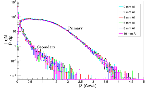
Figure 2: Momentum distribution of TOF points within STS and MuCh acceptance.
