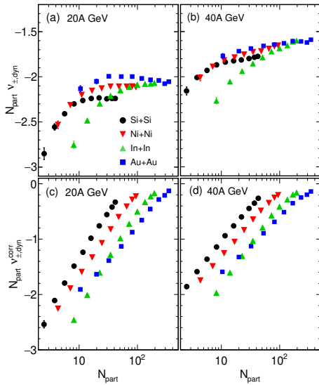
Figure 3: Centrality dependence of the dynamical net-charge fluctuations multiplied by the number of participating nucleons.
