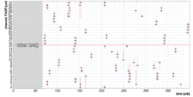
Figure 2: A 10 \mu\text{s} snap shot of signals' space-time dependence as delivered by TRD17/FASP/FASPRO at top rates obtained by x-rays bombardment.
