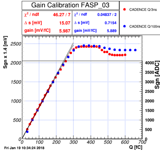
Figure 4: Electronic gain calibration of the FASP ASIC based on CADENCE™ simulations.
