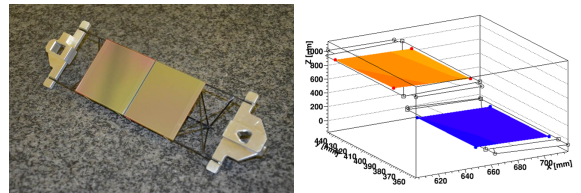
Figure 2: Two sensors glued onto a carbon fiber structure (left); Metrology of the mounted Sensors (right).
