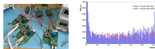
Figure 2: DPB boards for one test station (left); Measured noise with baby sensor (right).
