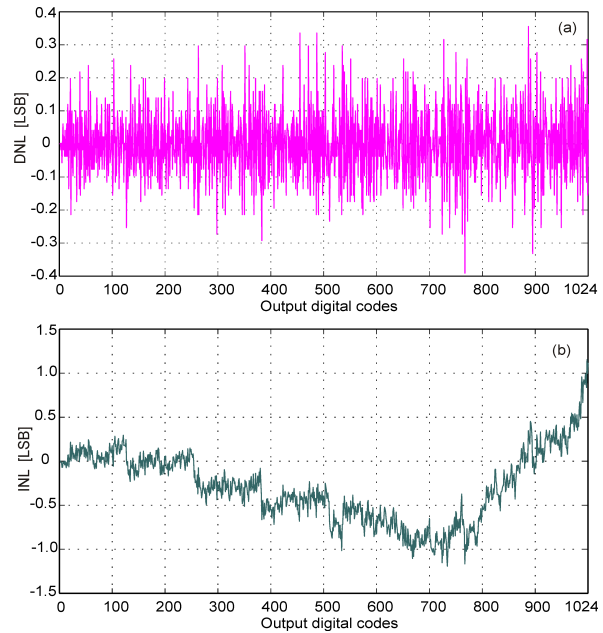
Figure 2: Measured typical static performance of ADC. (a) Differential non-linearity and (b) Integral non-linearity
