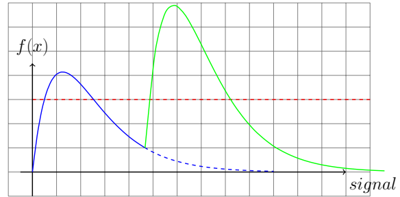
Figure 1: Diagram of a multi-hit-predecessor in blue and a follower in green. The red dashed line is the trigger threshold.
