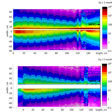
Figure 2: The ionizing energy loss at 10 AGeV for PSD with beam hole: 6 cm (upper picture) and 20 \times 20\ \text{cm}^2 (bottom picture) for horizontal cut.
