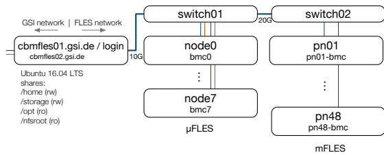
Figure 1: Architecture of the FLES development cluster including the newly acquired nodes. Only the Ethernet network used for file sharing and management is shown.
