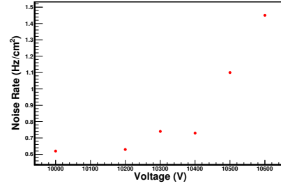
Figure 6: Noise Rate as a function of applied high voltage
