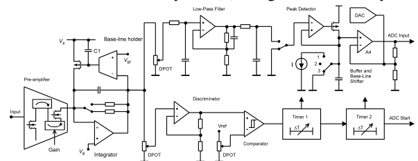
Figure 3: Functional diagram of one channel of analog ASIC
