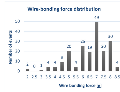
Figure 3: Measured bonding forces for the three malfunctioning sensors on the front side of the PRESTO module.
