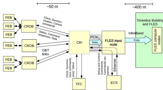
Figure 3: Schematics of the CBM data acquisition and processing system. Acronyms: FEB - Front End Board, CROB - Common Readout Board, CRI - Common Readout Interface, TFC - Timing & Fast Control, ECS - Experiment Control System, FLES - First Level Event Selector
