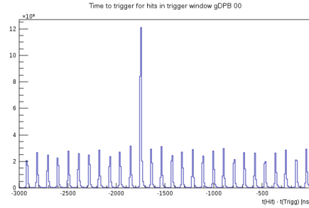
Figure 2: Time correlation between data driven by the MRPCs and the trigger signal generated by the STAR detector. An clear access at a time difference of about 1750 ns is visible.
