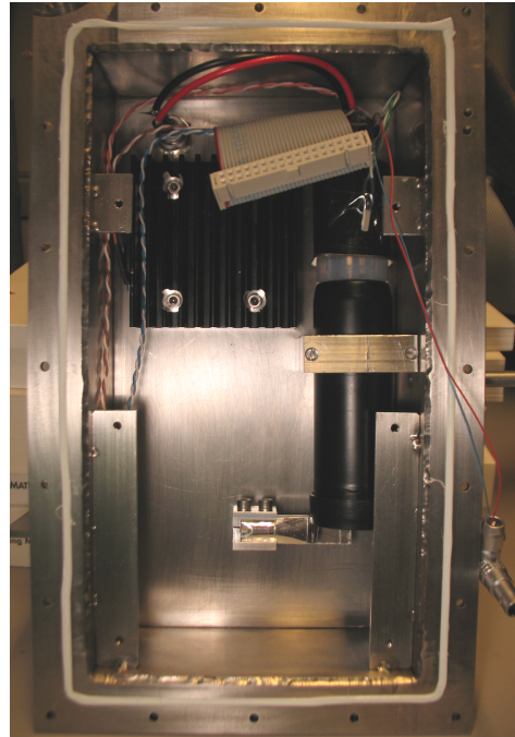
Figure 3: Photo of the sensor box with cooling fins, electrical feedthroughs and the PM tube with attached scintillator encased in reflective foil.
