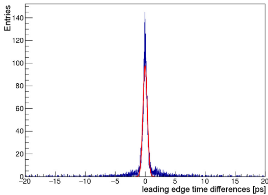
Figure 1: The leading-edge time difference of channel 5 to channel 4 of DiRICH 0x1215 (Threshold: 80 mV).
