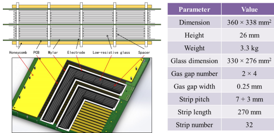
Figure 1: The structure and parameters of the CBM-ToF MRPC3a counter.
