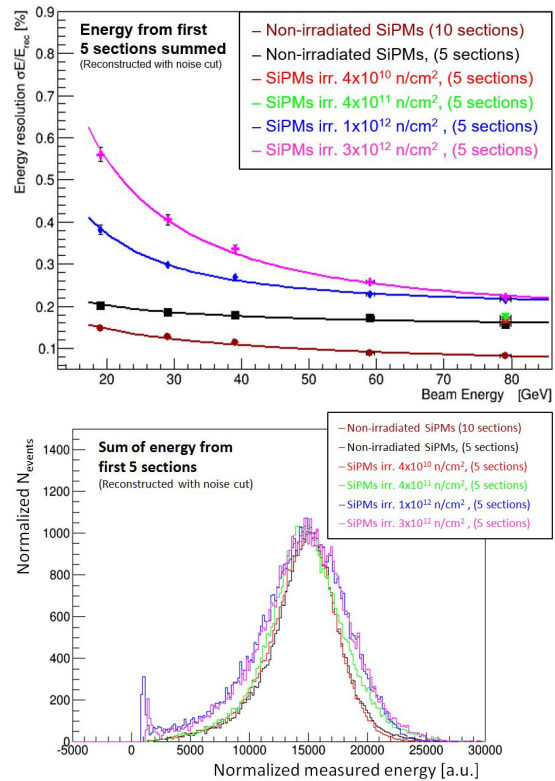
Figure 1: (top) Relative energy resolution measured for the proton beam energy scan from 20 up to 80 GeV. Half of NA61 PSD module was equipped with Hamamatsu SiPMs irradiated by neutrons with fluences in range from 4 \times 10^{10} up to 3 \times 10^{12} n/cm 2 . Energy resolution measured with all the 10 sections of module equipped with non-irradiated SiPMs is also shown for comparison in dark red (the lowermost curve). (bottom) Distribution of energy deposition in a single module for the 80 GeV/c proton beam.
