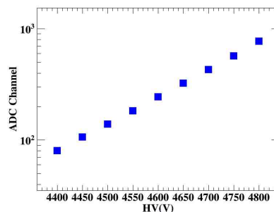
Figure 2: Linearity plot with respect to Voltage
