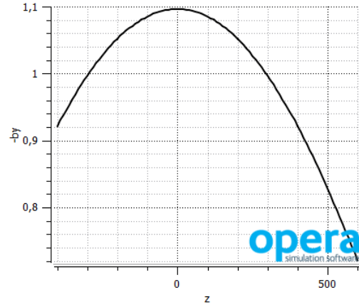
Figure 7: The vertical component of the magnetic field distribution for the muon version of the CBM detector. z position is given in \text{mm} .
