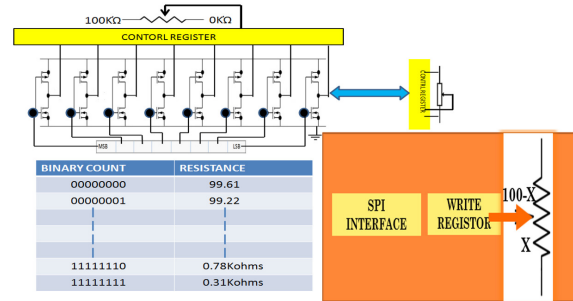
Figure 2: Layout of digital pot
