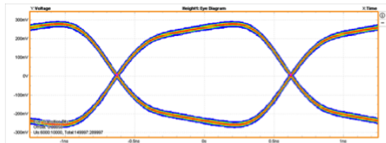
Figure 1: An eye diagram measured with DPO71254C Tektronix Oscilloscope at 400 MHz.
