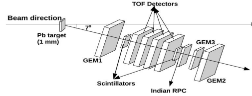
Figure 1: Schematic of experimental setup
