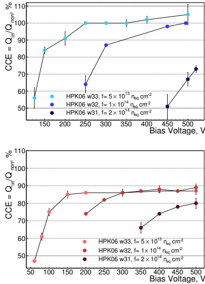
Figure 1: Charge collection as a function of the reverse bias voltage for p- and n-side (top and bottom plots, respectively) of 42 \times 62 \text{ mm}^2 HPK sensors.
