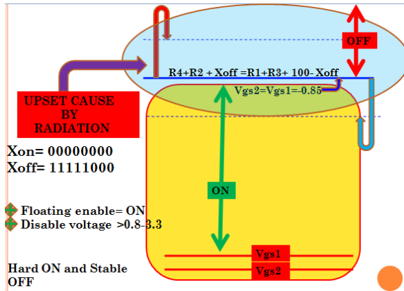
Figure 4: Effect of SEUs during OFF STATE
