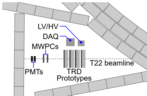
Figure 1: Floor plan of the setup at DESY. The beam is coming from the right. In the center the four large prototypes are shown.
