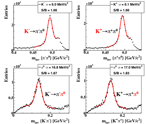
Figure 2: K^+ and K^- spectra obtained by the missing mass method together with their reconstructed \pi^0 neutral daughter particles using 700K mbias AuAu collisions at \sqrt{s_{NN}} = 200 GeV.
