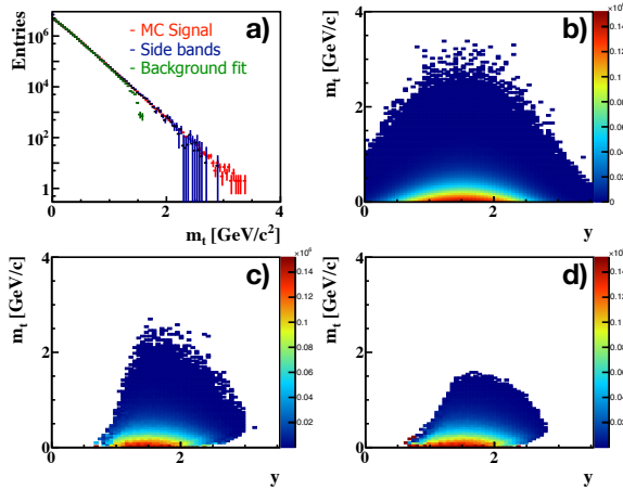
Figure 1: Efficiency corrected spectra of \Sigma^- hyperon as a function of a) m_t obtained by side bands and background fit methods with simulated signal; b) y-m_t for simulated signal; c) y-m_t by side band method; d) y-m_t by background fit.
