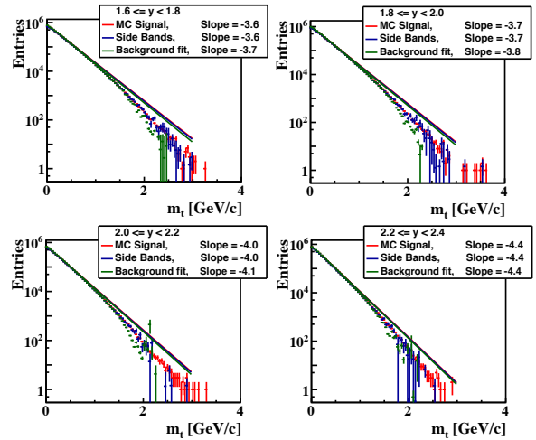
Figure 2: Reconstructed m_t signal in comparison to the simulated MC signal in different rapidity bins at an example of K_s^0 \rightarrow \pi^+\pi^- obtained from 5M central AuAu UrQMD events at 10 AGeV.
