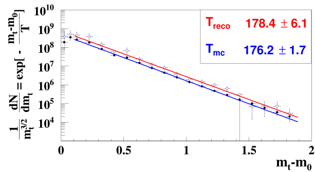
Figure 2: 1-dimensional p_t distributions of reconstructed \pi^0 after corrections (open circles) and simulated \pi^0 (full circles), fitted using formula 1.
