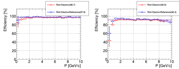
Figure 5: Ring reconstruction efficiency for primary electrons embedded in central Au+Au collisions. Left: 8A GeV, right: 25A GeV beam energy.
