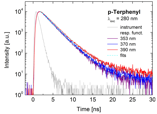
Figure 5: Normalized fluorescence intensity as a function of time after pulsed excitation at 280 nm for three different emission wavelengths. The dashed lines represent fits to the data (red, blue, and violet lines) taking into account two different decay constants and the measured instrument response function (grey line).
