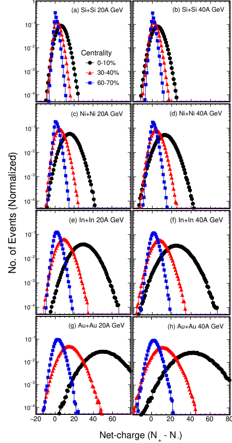
Figure 1: Distributions of event-by-event net-charge multiplicity within |\eta - \eta_0| < 1.0 at three centralities.
