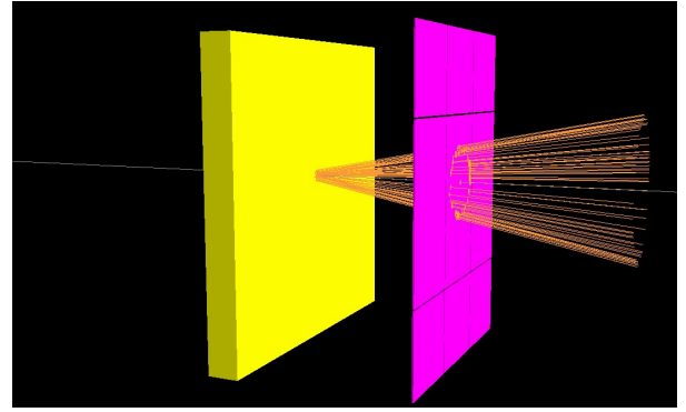
Figure 2: Event display of a single proton creating a RICH ring.
