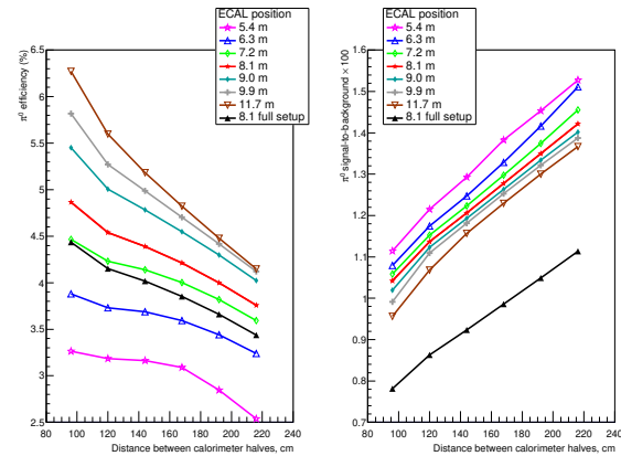
Figure 2: Neutral pion reconstruction efficiency (left plot) and signal-to-background ratio multiplied by factor 100 (right plot) as a function of distance between calorimeter halves and distance between target and calorimeter. 500K reconstructed events have been used for calorimeters located at 9 m and more from the target.
