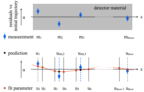
Figure 1: Top: Residuals versus initial trajectory along arc-length s . Bottom: Broken lines trajectory based on thin scatterers with offsets u .
