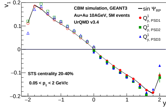
Figure 1: Directed flow of negatively charged pions for the 20-40% centrality class obtained using the y components of the PSD \mathbf{Q} -vectors. Shaded area corresponds to v_1 calculated using MC-true reaction plane. The open points have been reflected anti-symmetrically relative to zero rapidity.
