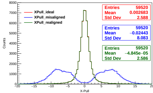
Figure 2: X-Pull distribution.
