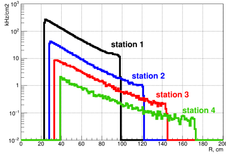
Figure 1: Particle Rate on the CBM-MUCH Stations in 10 AGeV minimum bias Au-Au collision
