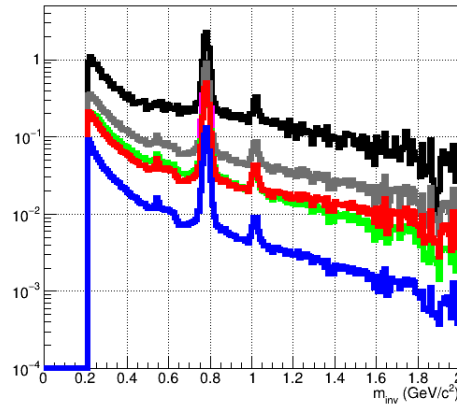
Figure 3: Signal-to-background ratio for muon pairs as function of invariant mass for central Au+Au collisions at 8 AGeV. Black: muon pairs from long tracks with ToF information, Grey: muon pairs from long-long and long-short tracks, both with ToF information, Red: muon pairs from long-long, long-short, and short-short tracks, both with ToF information, Green: muon pairs from long-long and long-short tracks, ToF information for long tracks only, Blue: muon pairs from long-long, long-short, and short-short tracks, ToF information for long tracks only.
