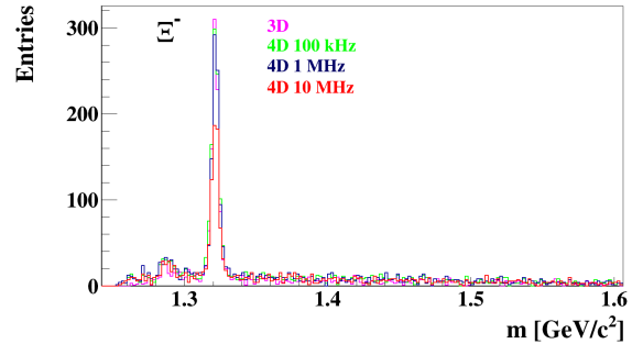
Figure 1: Invariant mass spectra of \Xi^- reconstructed in a time-slice with 0.5M minimum-bias Au+Au events at 10A GeV. Different interaction rate scenarios are shown with different colors.
