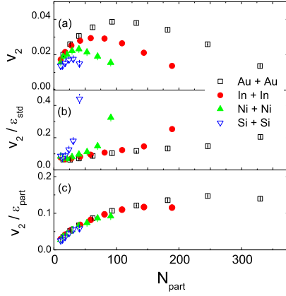
Figure 2: (a) Elliptic flow, (b) standard eccentricity ( \varepsilon_{\text{std}} ) scaled elliptic flow, and (c) participant eccentricity ( \varepsilon_{\text{part}} ) scaled elliptic flow of charged hadrons as functions of N_{\text{part}} at E_{\text{lab}} = 30A GeV.
