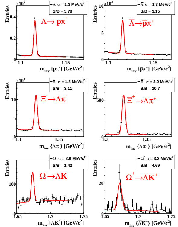
Figure 1: Reconstructed invariant-mass distribution of \Lambda , \bar{\Lambda} , \Xi^- , \bar{\Xi}^+ , \Omega^- , \bar{\Omega}^+ particles in Au+Au minbias collisions at \sqrt{s_{NN}} = 7.7 GeV, the red line indicates the signal plus background fit by a polynomial plus Gaussian function.
