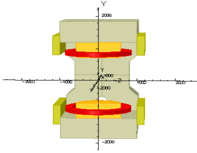
Figure 5: 3D model for the BINP design of the CBM SC dipole magnet.
