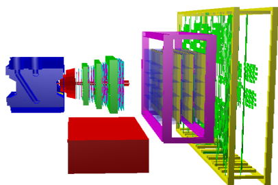
Figure 1: SIS100 CBM LMVM muon setup
