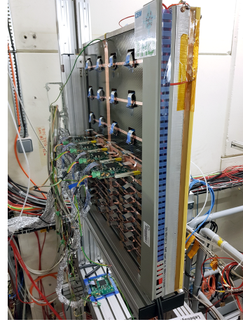
Figure 2: Experimental setup at GIF. A 2012-style MWPC prototype with four SPADIC 2.0 front-end boards.
