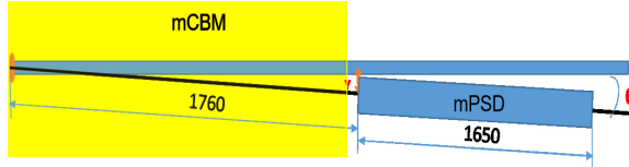
Figure 3: Schematic side view of the mPSD position at mCBM.
