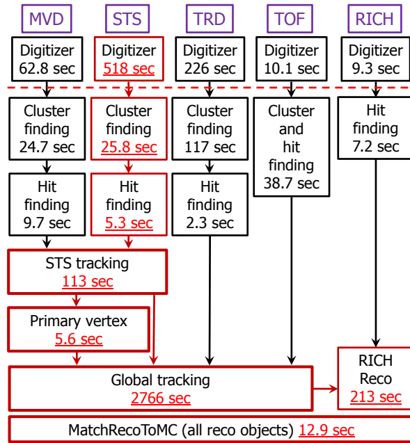
Figure 1: Flow graph of CbmRoot (digitisation plus reconstruction)
