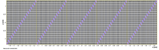
Figure 2: Track splitting in the x - y plane according to the read-out electrode geometry.
