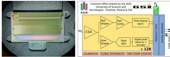
Figure 1: The STS/MUCH-XYTER ASIC and ASIC Configuration Diagram.
