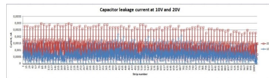
Figure 3: Capacitor leakage current at 10 and 20 V.
