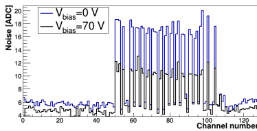
Figure 2: Noise of the setup: blue – 0 V; black – 70 V.
