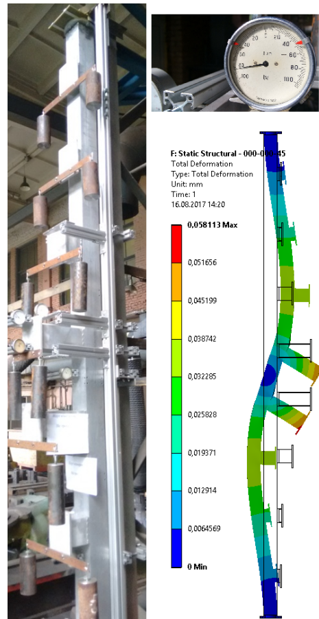
Figure 2: Test pillar under load (left). Micrometer used for measurements (upper right). Example of ANSYS deformation calculation (lower right).
