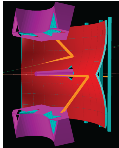
Figure 3: Event display of single electrons and their Cherenkov lightcone (orange) in the RICH detector.
