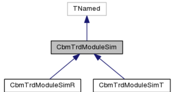
Figure 6: CbmRoot TRD module inheritance chart
