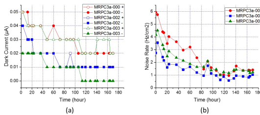
Figure 5: The dark current and noise rate of 3 MRPC3a counters monitored in 170 hours since HV training.
