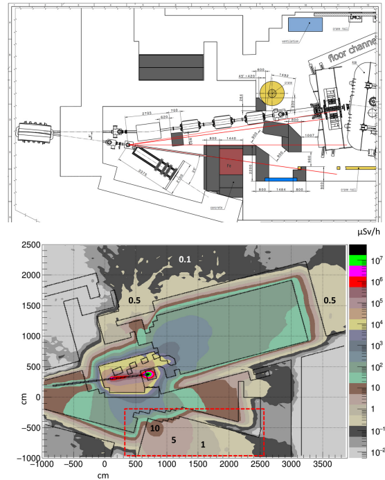
Figure 2: Top panel: the mCBM cave with additional concrete shielding (gray) and with the iron core of the mCBM beam dump (red). Bottom panel: corresponding FLUKA calculation (cross section = beam level), 10^8 Au ions \text{s}^{-1} at 1.24 AGeV on 10% interaction Au-target.
