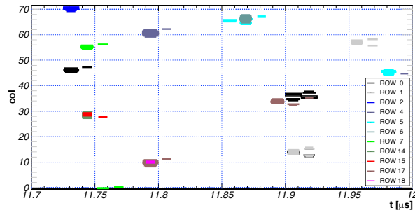
Figure 8: Time-based simulation with CbmRoot at 1 MHz interaction rate: distribution of digis in space-time for one Au+Au interaction seen in the mBUCH module
