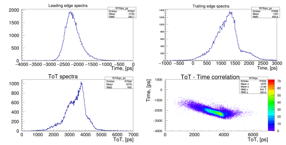
Figure 2: Spectra of leading (top-left) and trailing (top-right) edges, ToT (bottom-left) and ToT-Time correlation (bot-right) for cell 4 with field strength E=92 kV/cm and threshold set to 180 mV.
