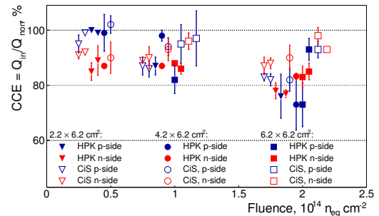
Figure 2: Charge collection efficiency for irradiated sensors from 5 \times 10^{13} 1 \text{ MeV } n_{\text{eq}} \text{ cm}^{-2} to 2 \times 10^{14} 1 \text{ MeV } n_{\text{eq}} \text{ cm}^{-2} .
