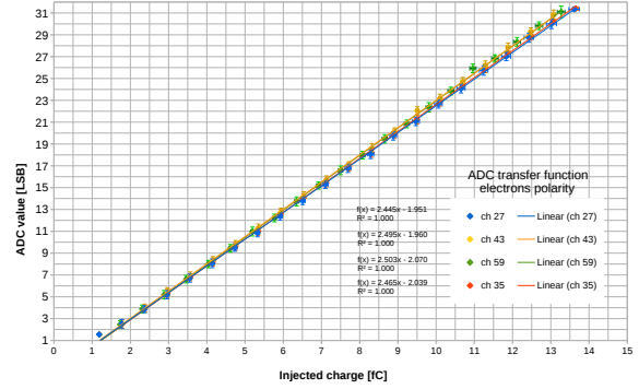
Figure 1: ADC response to negative injected charge pulses
