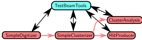
Figure 1: Dataflow in the new analysis framework. The data is processed in a pipeline of analysis classes (red boxes) and afterwards handed off to the next stage (red arrows). The analysis classes all call the TestBeamTools instance (teal box) to query the necessary parameters.
