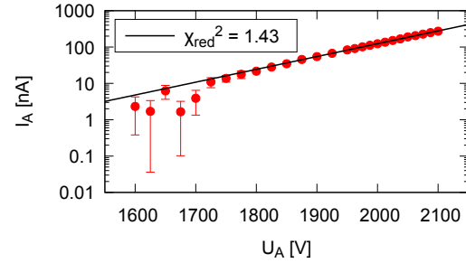
Figure 1: Anode current as a function of U_A , fit by I(U) = a \cdot \exp(b \cdot U)
