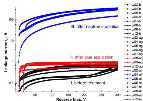
Figure 2: Current-voltage curves of sensors measured before treatment, after glue application and after irradiation.
