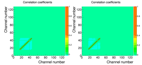
Figure 3: Correlation pattern for the single-metal sensor (left panel) and for the double-metal one (right panel) between all channel pairs.
