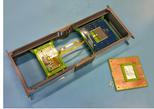
Figure 2: Partially equipped STS module S^2M01 . The sensor n-side cover is removed to show the 42 \times 62 \text{ mm}^2 sensor with the attached micro-cables.
