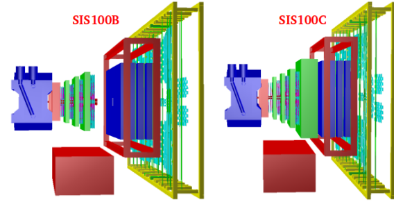
Figure 3: Muon detection system with 4 stations + 4 absorbers (SIS100B) (left) and 5 stations + 5 absorbers (SIS100C) (right).
