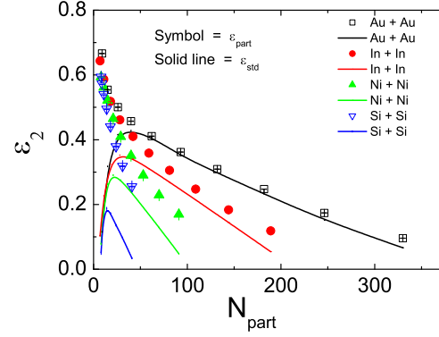
Figure 1: Eccentricity as a function of N_{part} for various heavy-ion collisions at E_{lab} = 30A GeV.
