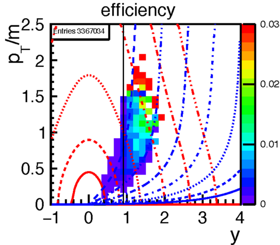
Figure 9: Efficiency of reconstructed \Lambda - baryons with mCBM produced in Ni + Ni collisions at 1.93 AGeV (input: events generated with UrQMD). Red and blue lines indicate constant laboratory momenta and laboratory polar angles, respectively. The black line indicates mid-rapidity.
