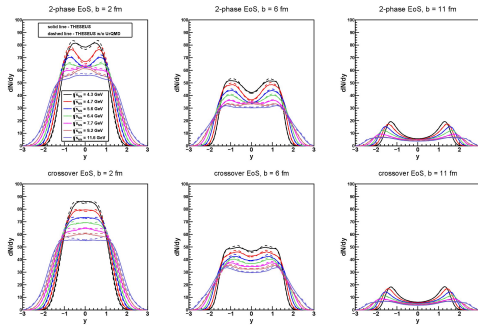
Figure 1: Proton rapidity distribution for Au+Au collisions for different EoS, energies and impact parameters from [1].
