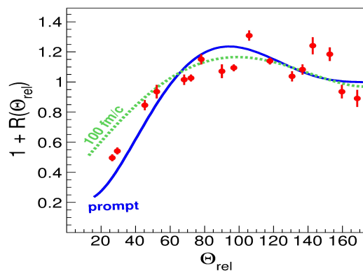
Figure 1: Relative angle correlation function for IMF produced in {}^4\text{He} + \text{Au} collisions at 4 GeV. Lines are explained in the text.
