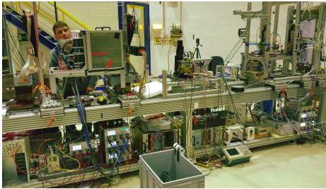
Figure 1: Photograph of the joined COSY test beam setup Nov. 2017
