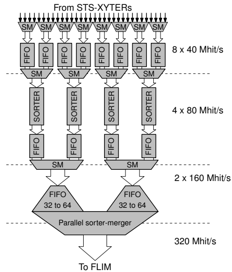
Figure 1: Structure of the data concentration system developed for stsDPB (SM - simple mergers).
