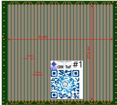
Figure 1: MRPC3b counter with QR sticker.
