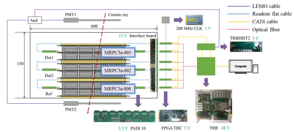
Figure 6: The diagram of the cosmic test system based on TRB board, FPGA TDC and PADI10 front-end electronics.
