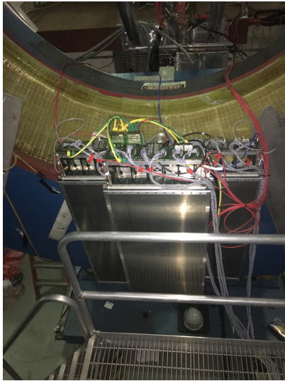
Figure 4: One sector mounted on the inner side of the pole tip.
