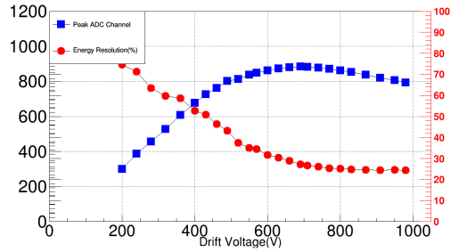
Figure 3: Variation of ADC and energy resolution with drift voltage
