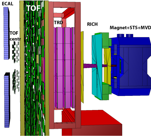
Figure 1: Cbmroot model of the CBM detector used in simulation.
