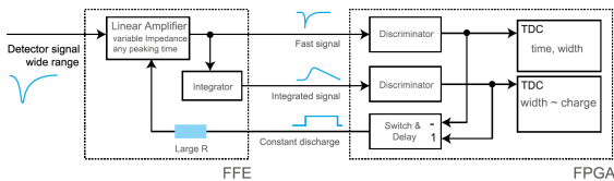
Figure 5: Logic layout of PaDiWa.
