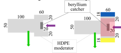
Figure 1: By simulations optimized moderator (left) and addition of material during the experiment (right).
