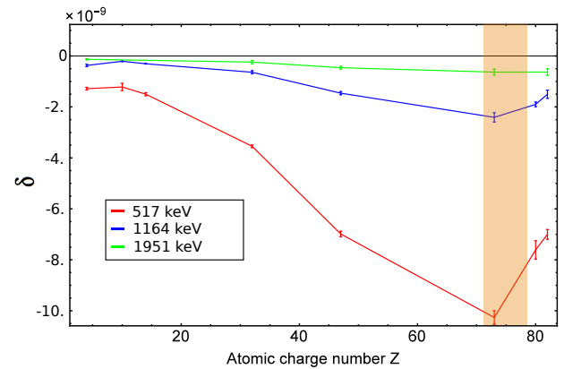
Figure 2: Z dependence of the measured \delta for three different photon energies. The shaded area highlights the range of materials with maximum mass density.
