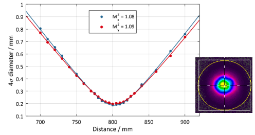
Figure 2: Beam caustic and output beam profile at 1.9kW average power proving a diffraction limited beam quality.
