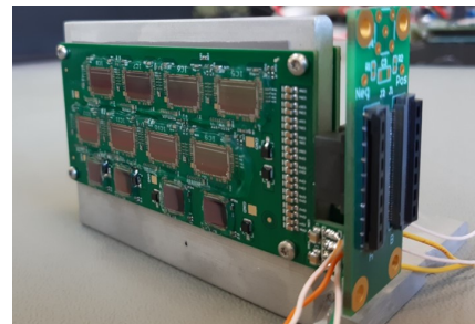
Figure 2: Two FEBs with a FEB-panel
