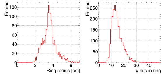
Figure 6: Left: ring radius distribution of reconstructed rings. Right: Number of hits in ring.
