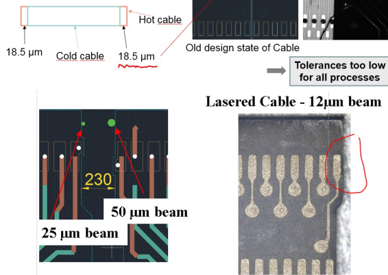
Figure 3: Top: The CTE and the small nominal gap between two adjacent cables of version v7 interferes with the soldering process of the cables on the sensor. Left: The design of the cable v8 with a larger gap for laser-singulation of the cables. Right: A well laser-singulated cable of version v8.
