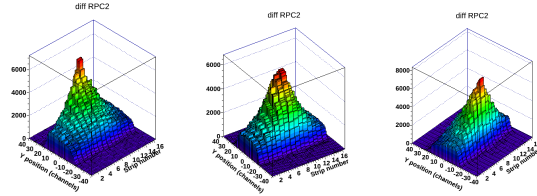
Figure 4: 3D - plots for the exposure of the active area to a collimated ^{60}\text{Co} source for up (left), center (middle) and down (right) positions along the strip.
