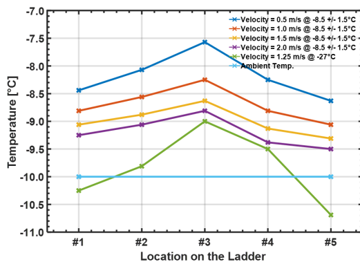
Figure 1: Variation of temperature along the ladder for different air-flow velocities and temperatures.
