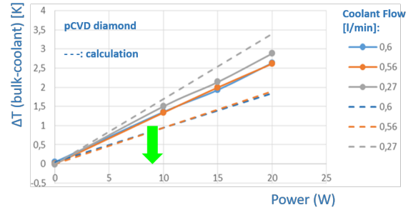
Figure 2: Measured (symbols) and calculated (dashed lines) temperature difference between heat converter bulk and coolant (Glycol:water = 1:1) for different flows. Temperature at point A (Fig.1) = -10^\circ \text{C} . Green arrow: MVD operation region.
