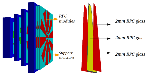
Figure 1: Arrangement of modules in staggered manner on both sides of a support structure. RPC module has been shown separately.
