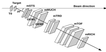
Figure 1: Schematics of the experimental setup of mCBM experiment for Nov./Dec.19 runs
