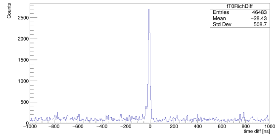
Figure 2: Timing distribution of the digis between T0 and mRICH after application of a time correction.
