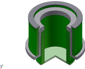
Figure 2: The structural model of a G-10 strut.
