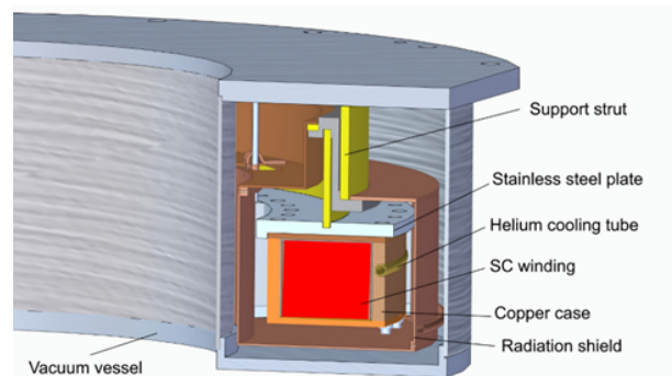
Figure 3: Cross section of the upper coil with the SC winding inside the copper case and the Helium cooling tube, the stainless steel plate the support strut, the radiation shield and the vacuum vessel.
