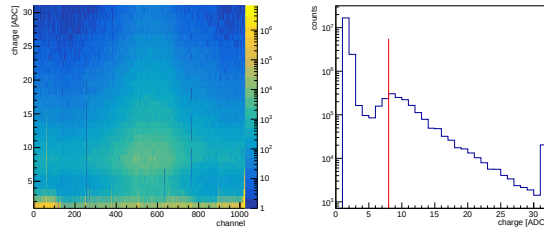
Figure 6: Beam profile seen in the channels of one sensor side (left), and signal distribution in one ASIC (right), all in ADC units before calibration.
