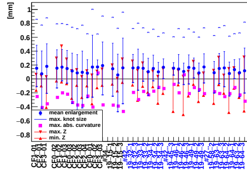
Figure 2: Metrology of 20% of the produced ladders.
