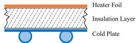
Figure 2: Cross-sectional schematic of the insulation panel.
