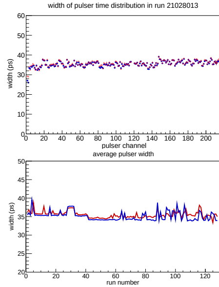
Figure 2: Upper plot: width of the time distribution obtained by measuring the arrival time of injected pulser signals on every GET4 board. Lower plot: mean of the time distribution width vs. the run number.
