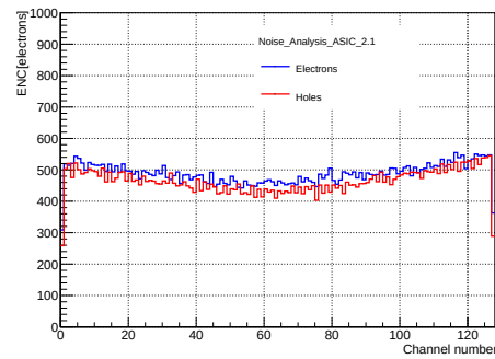
Figure 3: Noise for a single ASIC in prototype FEB-C.
