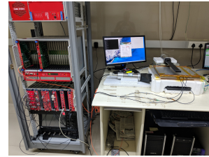
Figure 2: Picture of the RPC under test with electronics.
