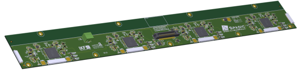
Figure 2: Rendering of the quad SPADIC 2.2 FEB used at mCBM.
