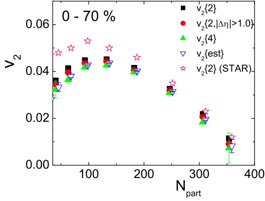
Figure 1: (Color online) v_2 as a function of N_{\text{part}} in Au+Au collision at E_{\text{lab}} = 30A GeV.
