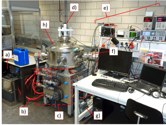
Figure 1: The test setup at IKF (GUF) named "UFO": a) HUBER cooling system, b) cooling pipes, c) distribution and control panel, d) IR camera, e) steering and R/O electronics, f) turbo molecular pump, g) scroll pump, h) vacuum chamber.
