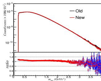
Figure 4: Di-muon invariant mass spectra of the combinatorial background for central Au+Au collision at 8A GeV with different configurations of the first absorber.
