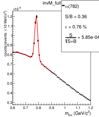
Figure 3: Invariant mass distribution with 60 cm-20 cm-20 cm-30 cm absorber configuration. One \omega has been embedded per event.
