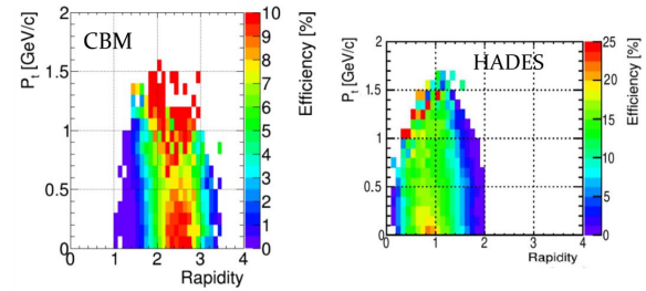
Figure 3: P_t -y coverage of calculated efficiencies for the \omega -meson. For HADES we see efficiencies up to 20% at midrapidity ( y_{CM}=1.13 ) while CBM has a higher efficiency in forward rapidity.
