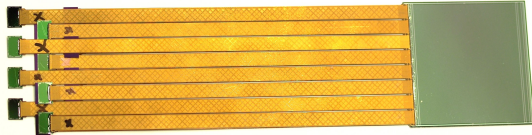
Figure 8: First copper module completely assembled with STS-XYters on N- and P-side.
