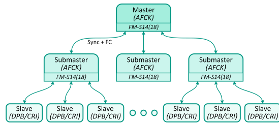
Figure 1: TFC system topology.
