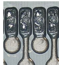
Figure 6: Perfectly centered imprints of the Au stud bumps from the sensor side in the solder depot of the cable.
