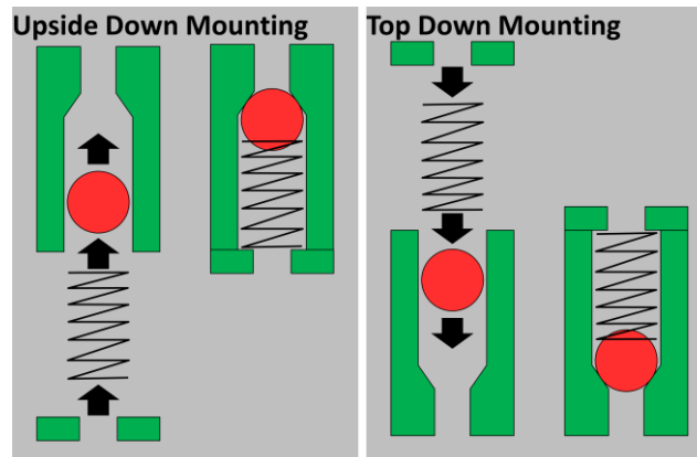
Figure 272: DFMA Upside Down Mounting (Image Roser)
