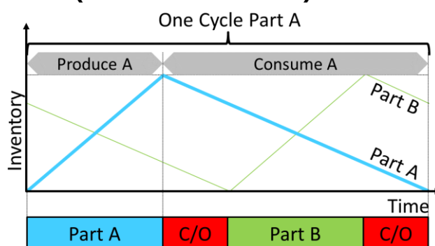
Figure 465: Inventory subject to changeover: two parts, one cycle (Image Roser)
