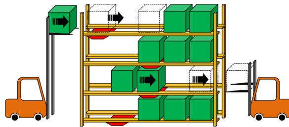
Figure 94: Radio Shuttle Storage (Image Roser)
