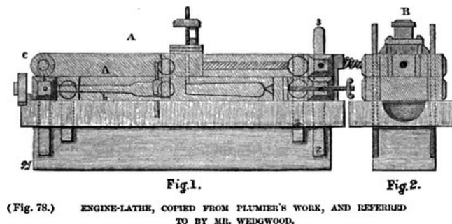
Figure 11: Lathe used in the Wedgwood Factory (Image Eliza Meteyard in public domain)
