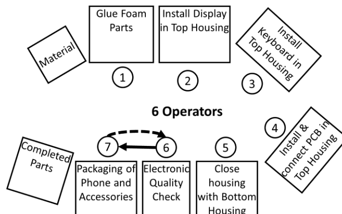
Figure 50: Flexible Manpower Example Layout 6 Operators (Image Roser)
