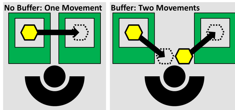
Figure 436: Chaku Chaku Buffer (Image Roser)
