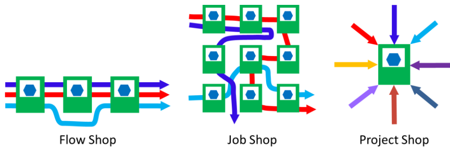
Figure 30: Flow Shop Job Shop Project Shop (Image Roser)
