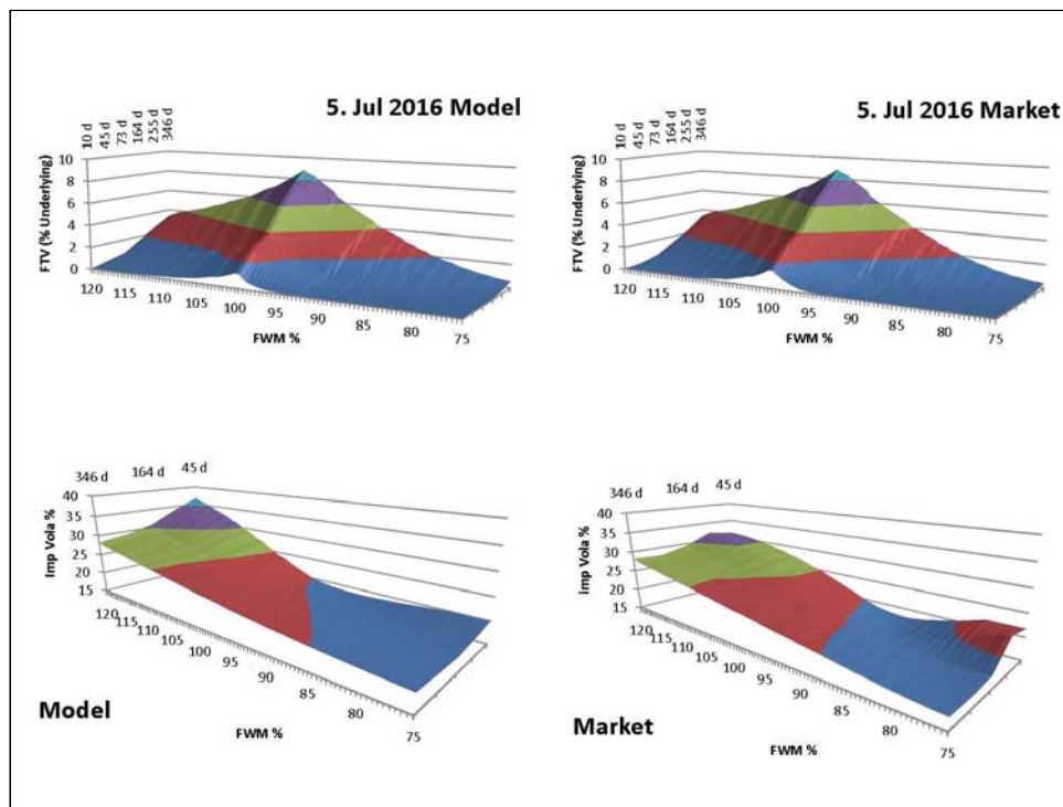
3D charts: forward time value (FTV) and implied volatility surface (IVS)
