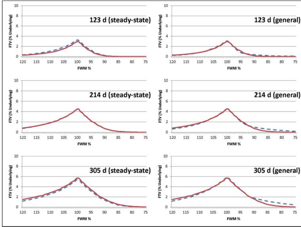
Comparison best steady-state and best general augmented model (part 2)
