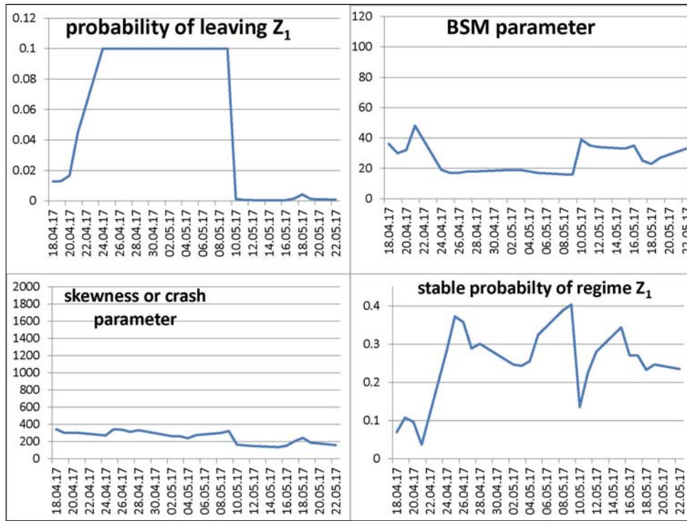
Parameters or related values of the best detected general models (French election)
