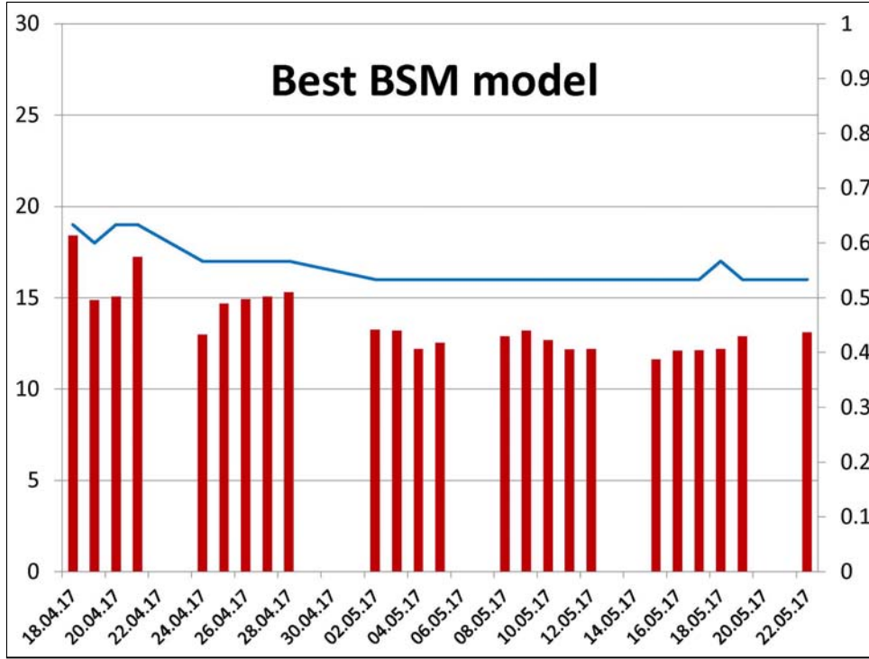
Best BSM model: volatility parameter and norm distance to market prices
