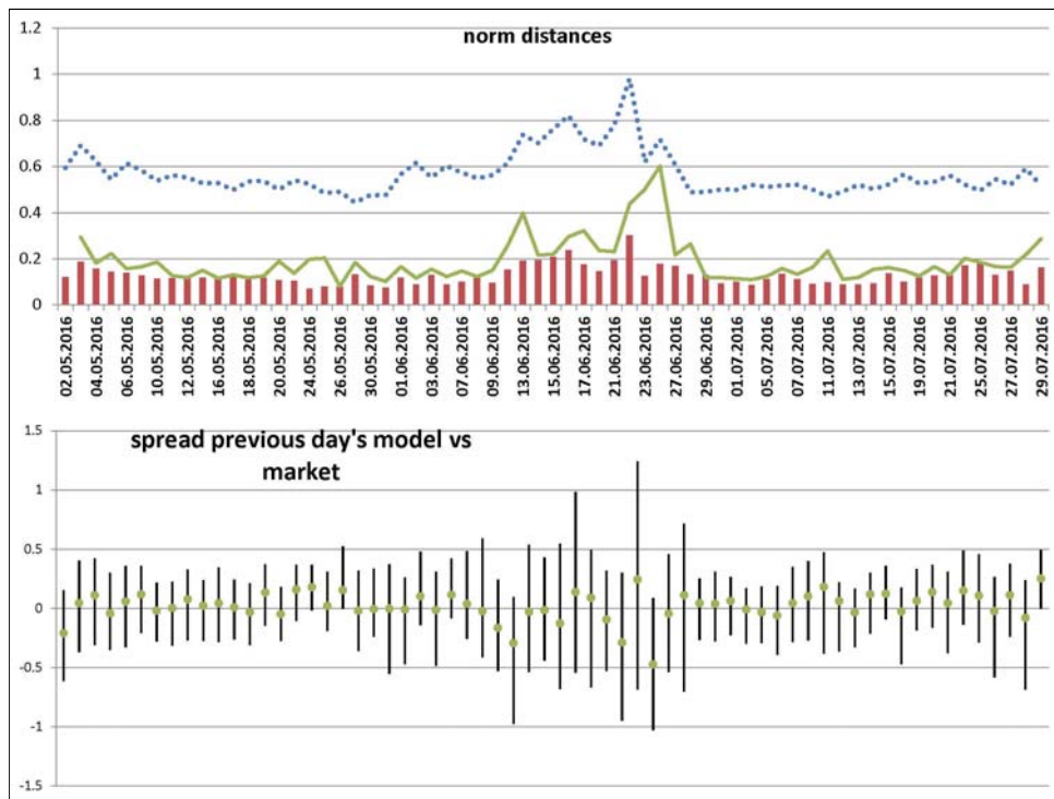
Norm distances and spreads in context with “yesterday’s model” (see text)
