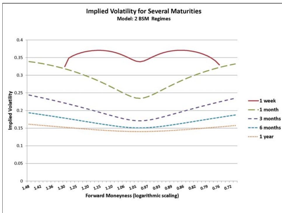
Smiles of a general augmented 2 BSM regimes model
