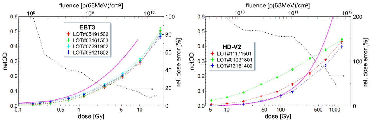
Fig. 1: Dose response of EBT3 (left) and HD-V2 (right) for films from different production batches. For comparison, the solid (magenta) curves show previous calibrations of EBT3 [3] and HD810 ([4], Kodak Wratten 94 filter), the predecessor to HD-V2. The dash-dotted (black) curve shows the relative dose error due to the variability of the response curve.
