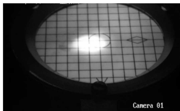
Fig.2. The beam spot after the acceleration tube.
