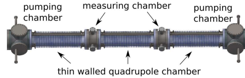
Figure 1: Prototype quadrupole chamber setup
