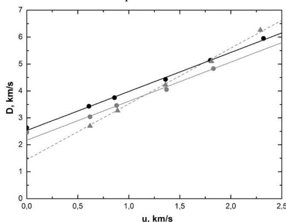
Figure 1: Hugoniot parameters of kevlar and textolite.
