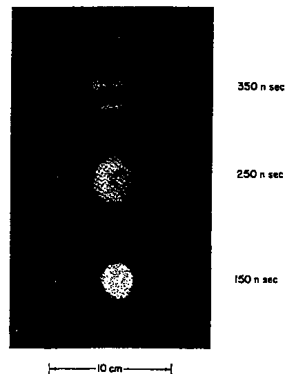
Fig. 1. Side-on framing camera picture of a plasma produced from an aluminum sphere of 80 \mu\text{m} radius at the time indicated after irradiation from the left hand side by a 30 ns ruby laser pulse focused to 0.4 mm diameter at the mentioned times after irradiation. The second frame shows the outer part of a rapidly expanding half-moon-like plasma and an inner spherical thermally expanding part [5]
