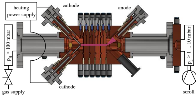
Figure 1: Schematic and cross section of the experimental setup with heating power supply
