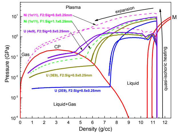
Figure 2: pressure-density phase diagram of Lead
