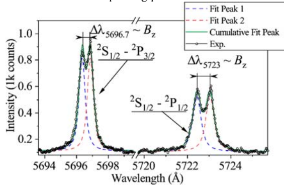
Figure 1: Spectral lines of Al III 4s - 4p ( \lambda = 5696.6 -Å and 5722.7-Å) from laser dopant plasma, recorded at t = -115 ns from stagnation ( t = 0 ), z = 7 mm ( z = 0 is anode-nozzle surface). Zeeman splitting pattern is clearly observed. From peak separation of individual Al III transitions, proportional to B_z , it is obtained B_z = (1.6 \pm 0.1) T.
