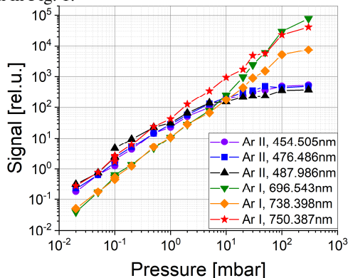
Figure 1: Pressure dependence of the intensity of selected atomic and ionic argon lines excited by a 85 MeV ^{32}\text{S} beam.
